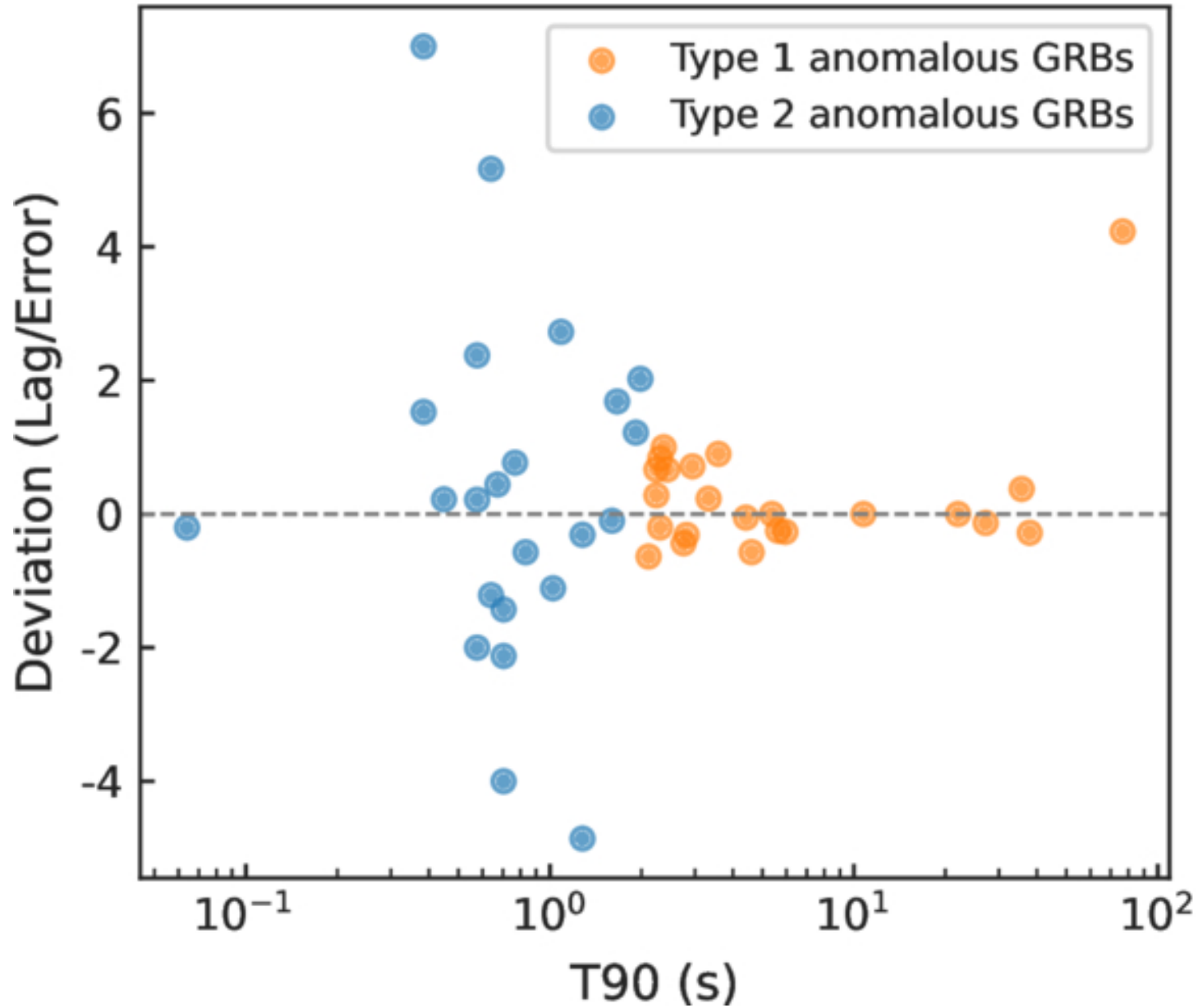
Figure 4. from Shi-Qi Wei et al 2026 Astrophys. J. Lett. 1003 doi:10.3847/2041-8213/ae67f9 https://dx.doi.org/10.3847/2041-8213/ae67f9 © 2026. The Author(s). Published by the American Astronomical Society.
