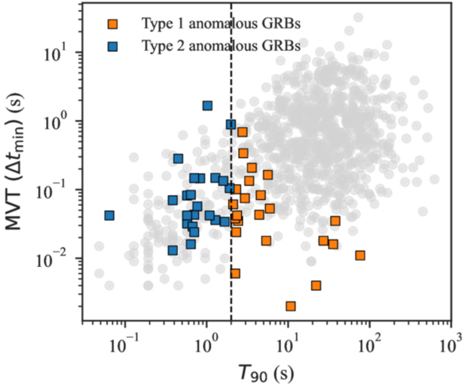
Figure 2. from Shi-Qi Wei et al 2026 Astrophys. J. Lett. 1003 doi:10.3847/2041-8213/ae67f9 https://dx.doi.org/10.3847/2041-8213/ae67f9 © 2026. The Author(s). Published by the American Astronomical Society.
