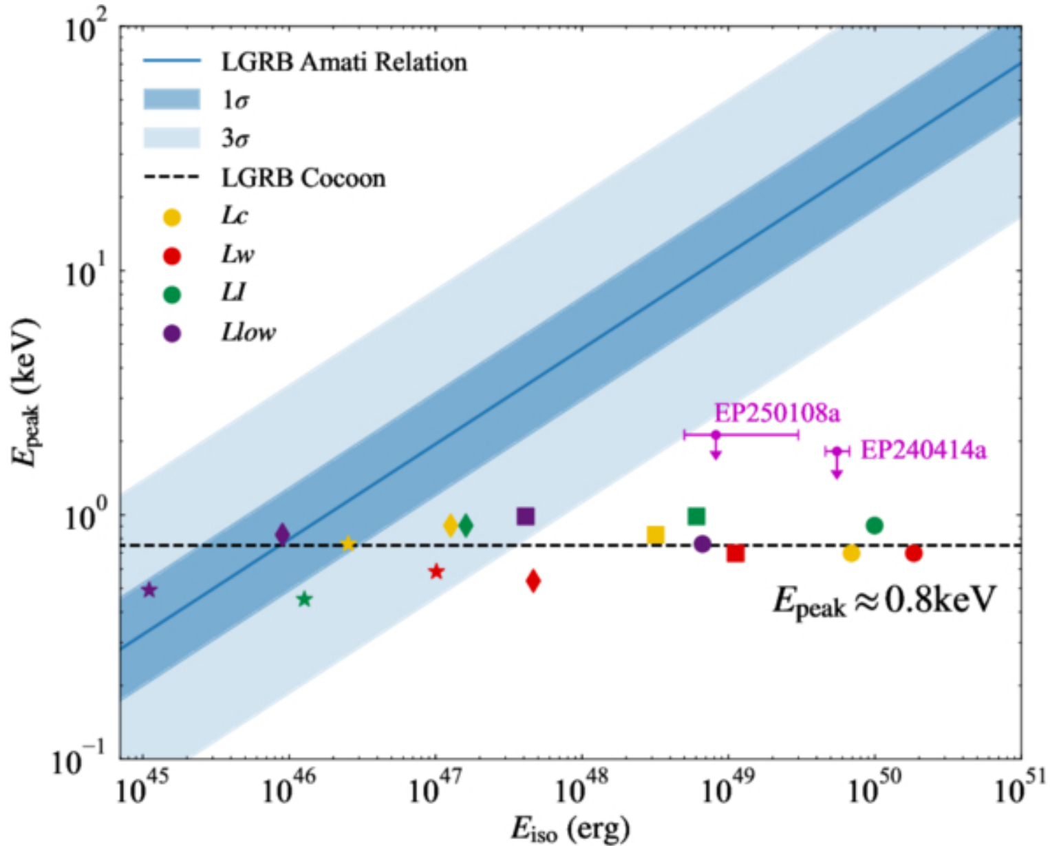
Figure 9. from Jian-He Zheng and Wenbin Lu 2026 Astrophys. J. Lett. 1003 doi:10.3847/2041-8213/ae67f2 https://dx.doi.org/10.3847/2041-8213/ae67f2 © 2026. The Author(s). Published by the American Astronomical Society.
