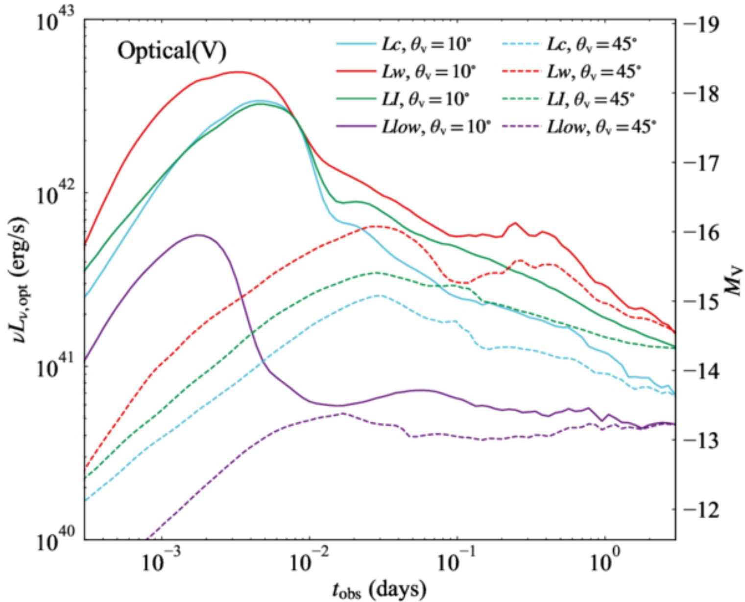
Figure 13. from Jian-He Zheng and Wenbin Lu 2026 Astrophys. J. Lett. 1003 doi:10.3847/2041-8213/ae67f2 https://dx.doi.org/10.3847/2041-8213/ae67f2 © 2026. The Author(s). Published by the American Astronomical Society.
