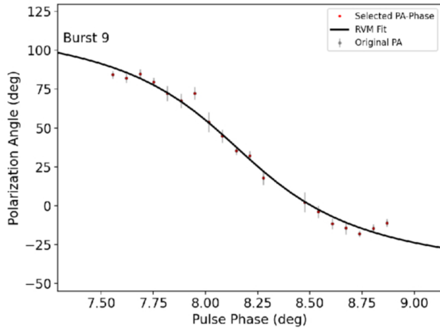
(a) Burst 9: RVM fit for the central phase region.
