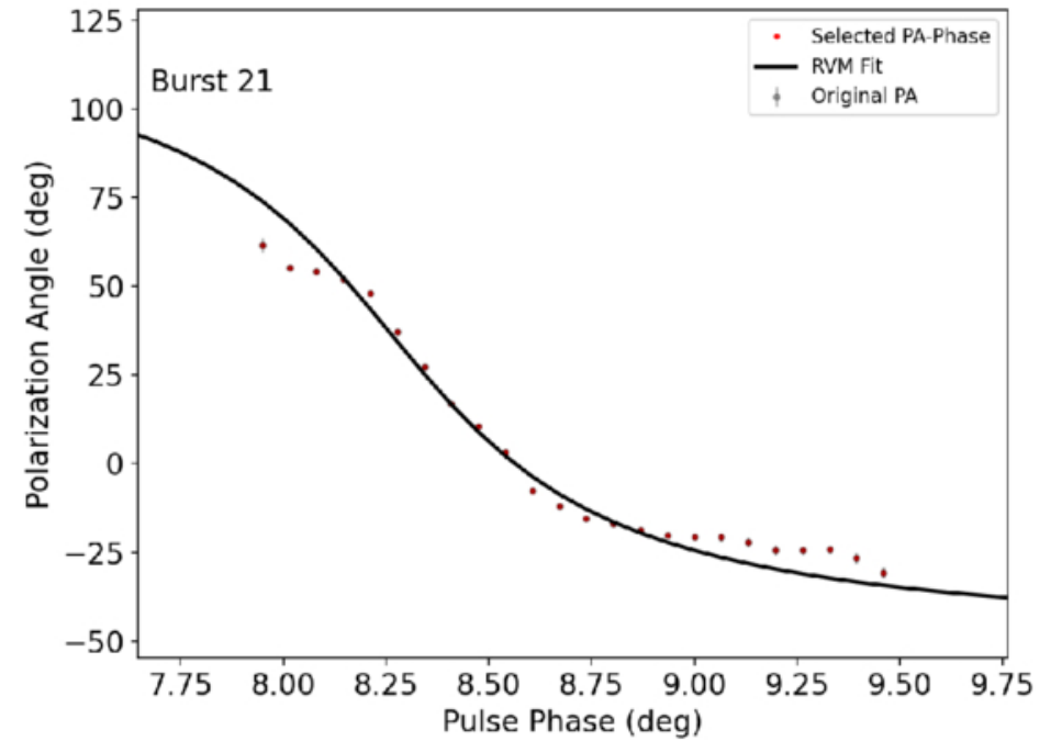
(b) Burst 21: RVM fit for the trailing phase region.
