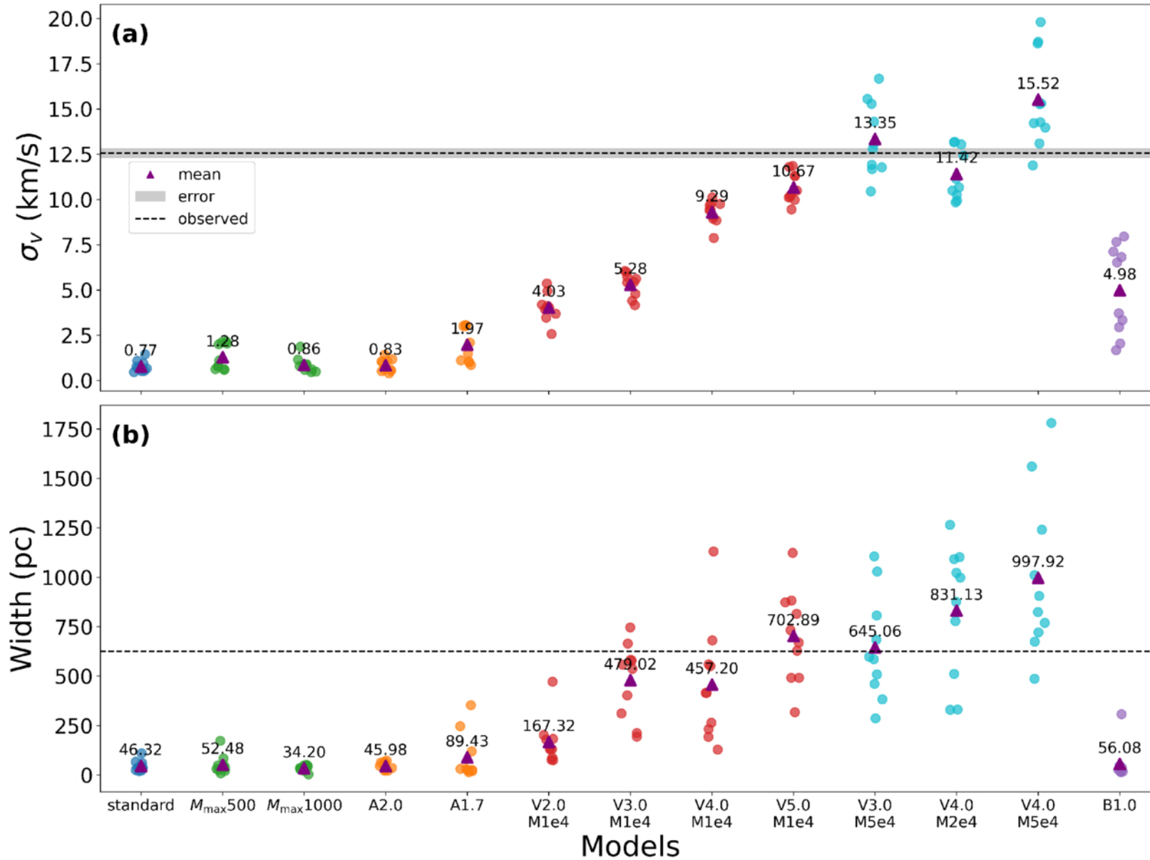
Figure 2. from Zhen Wang et al 2026 Astrophys. J. Lett. 1003 doi:10.3847/2041-8213/ae67ee https://dx.doi.org/10.3847/2041-8213/ae67ee © 2026. The Author(s). Published by the American Astronomical Society.
