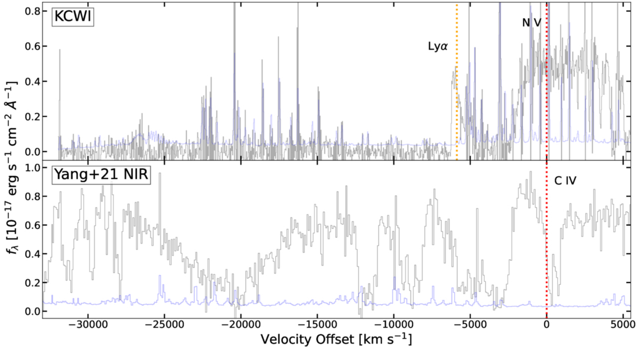
Figure 5. from Raymond P. Remigio et al 2026 Astrophys. J. Lett. 1003 doi:10.3847/2041-8213/ae67ed https://dx.doi.org/10.3847/2041-8213/ae67ed © 2026. The Author(s). Published by the American Astronomical Society.
