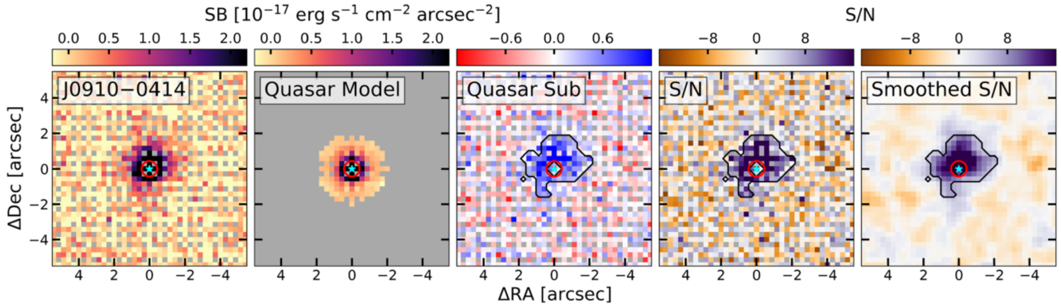
Figure 1. from Raymond P. Remigio et al 2026 Astrophys. J. Lett. 1003 doi:10.3847/2041-8213/ae67ed https://dx.doi.org/10.3847/2041-8213/ae67ed © 2026. The Author(s). Published by the American Astronomical Society.
