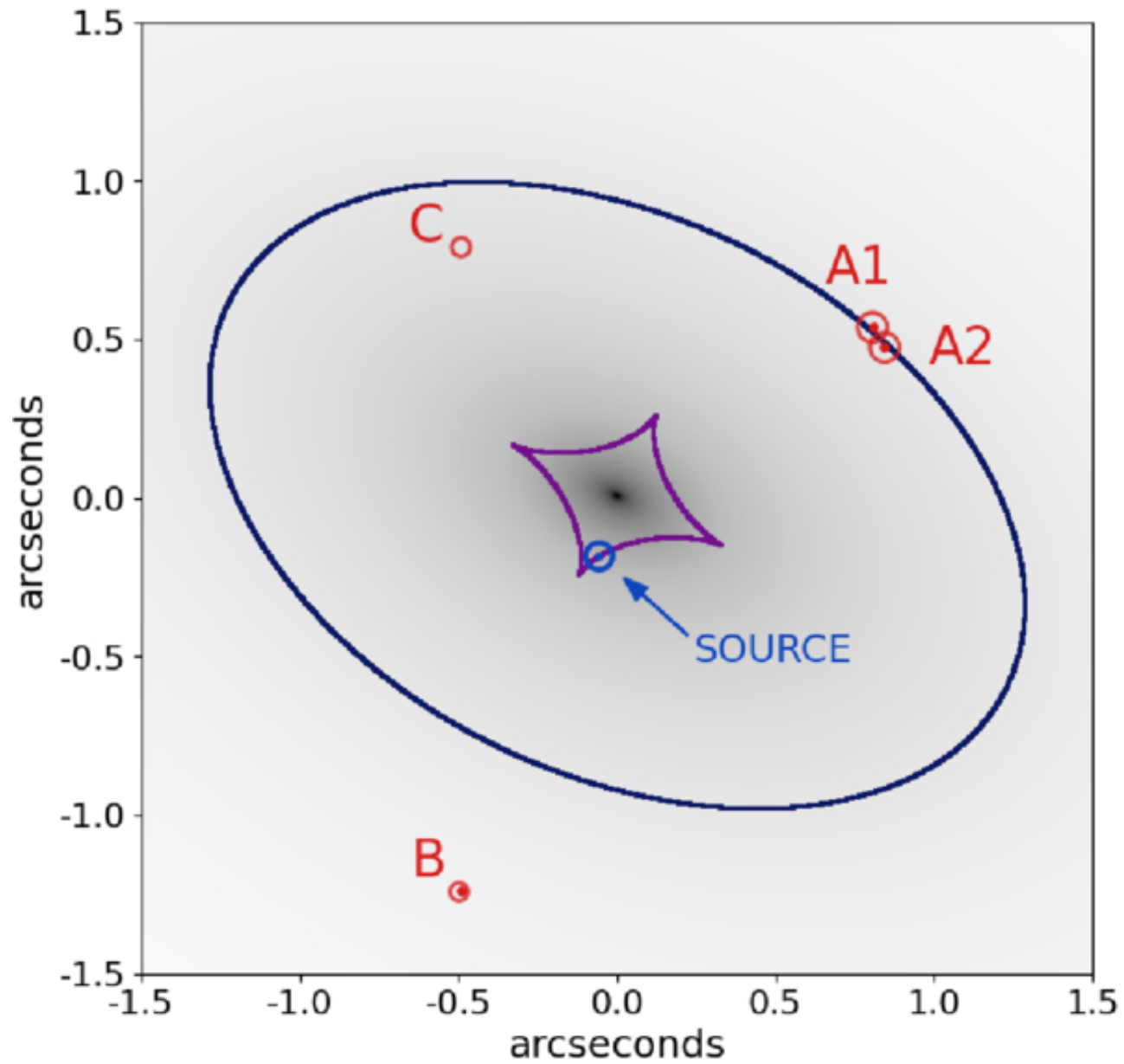
Figure 4. from Cameron Lemon et al 2026 Astrophys. J. Lett. 1003 doi:10.3847/2041-8213/ae6780 https://dx.doi.org/10.3847/2041-8213/ae6780 © 2026. The Author(s). Published by the American Astronomical Society.
