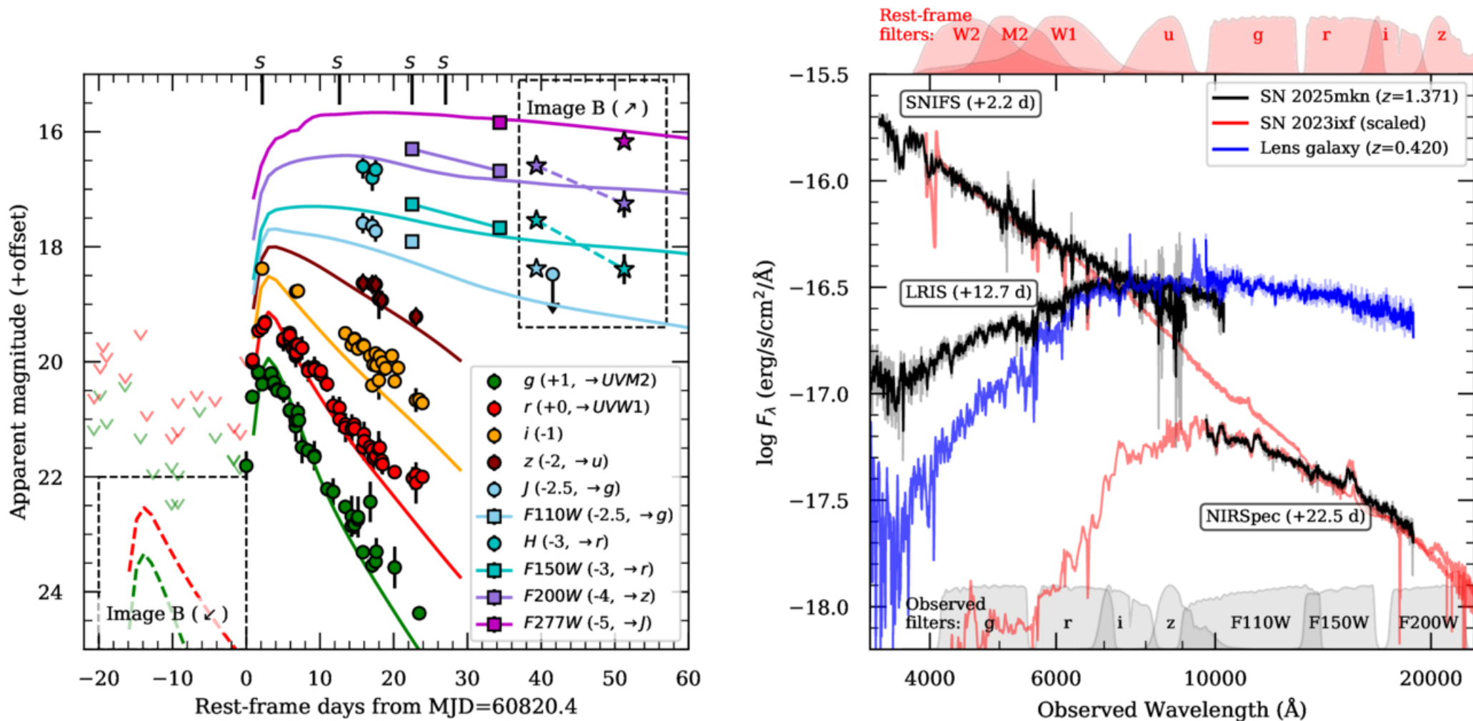
Figure 2. from Cameron Lemon et al 2026 Astrophys. J. Lett. 1003 doi:10.3847/2041-8213/ae6780 https://dx.doi.org/10.3847/2041-8213/ae6780 © 2026. The Author(s). Published by the American Astronomical Society.
