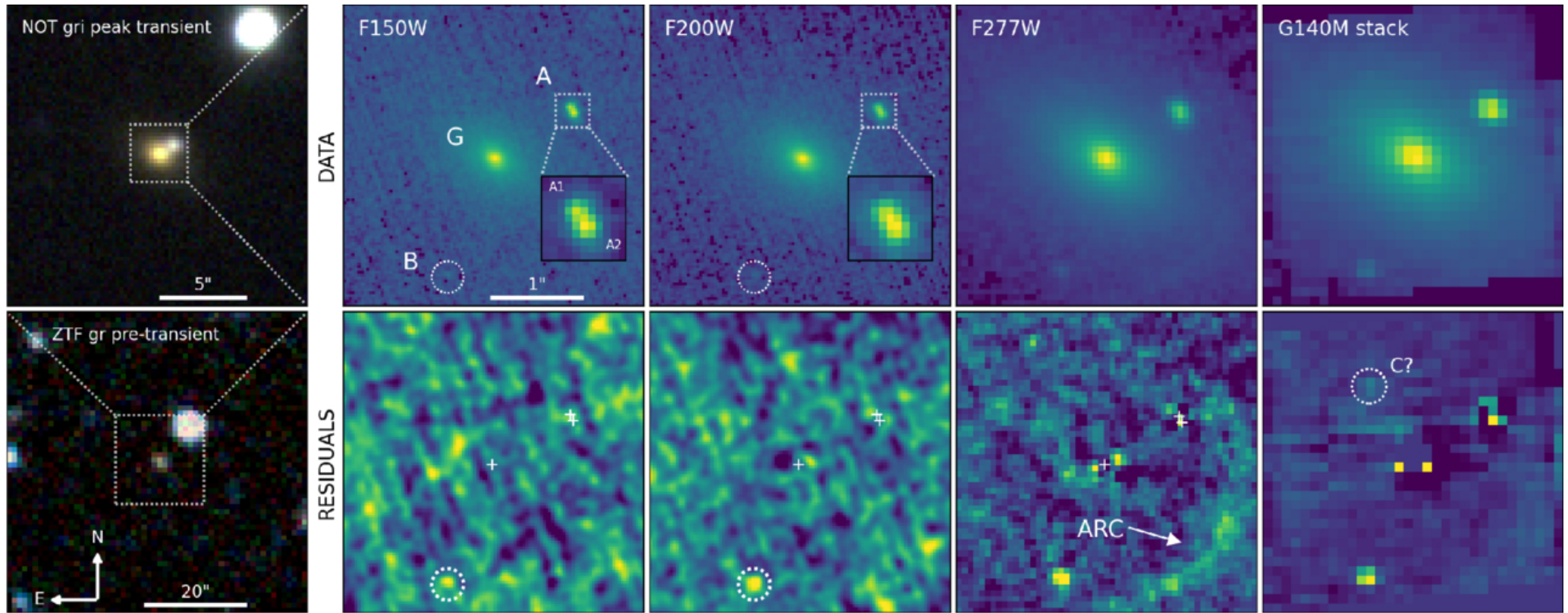
Figure 1. from Cameron Lemon et al 2026 Astrophys. J. Lett. 1003 doi:10.3847/2041-8213/ae6780 https://dx.doi.org/10.3847/2041-8213/ae6780 © 2026. The Author(s). Published by the American Astronomical Society.
