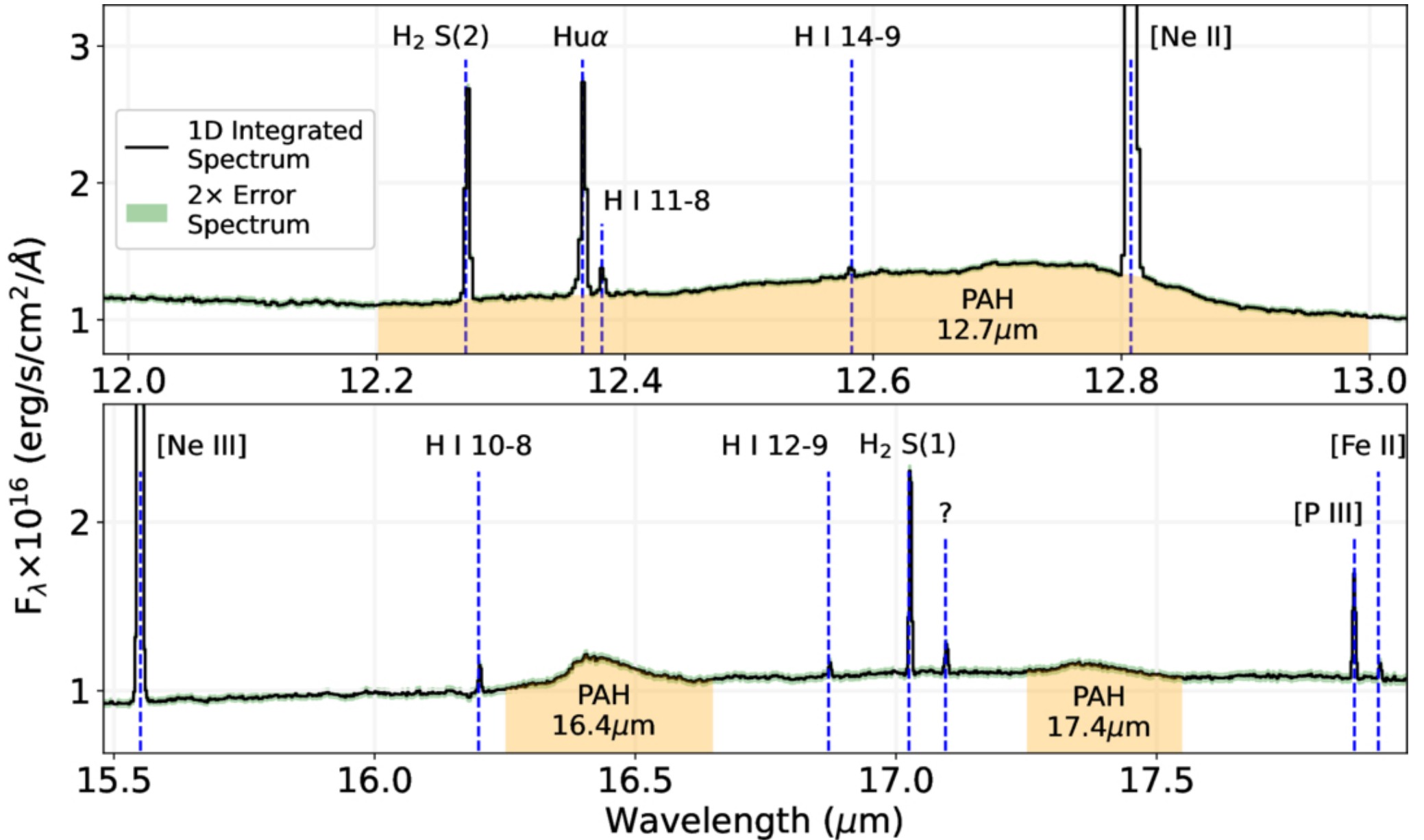
Figure 2. from Noah S. J. Rogers et al 2026 Astrophys. J. Lett. 1003 doi:10.3847/2041-8213/ae66f0 https://dx.doi.org/10.3847/2041-8213/ae66f0 © 2026. The Author(s). Published by the American Astronomical Society.
