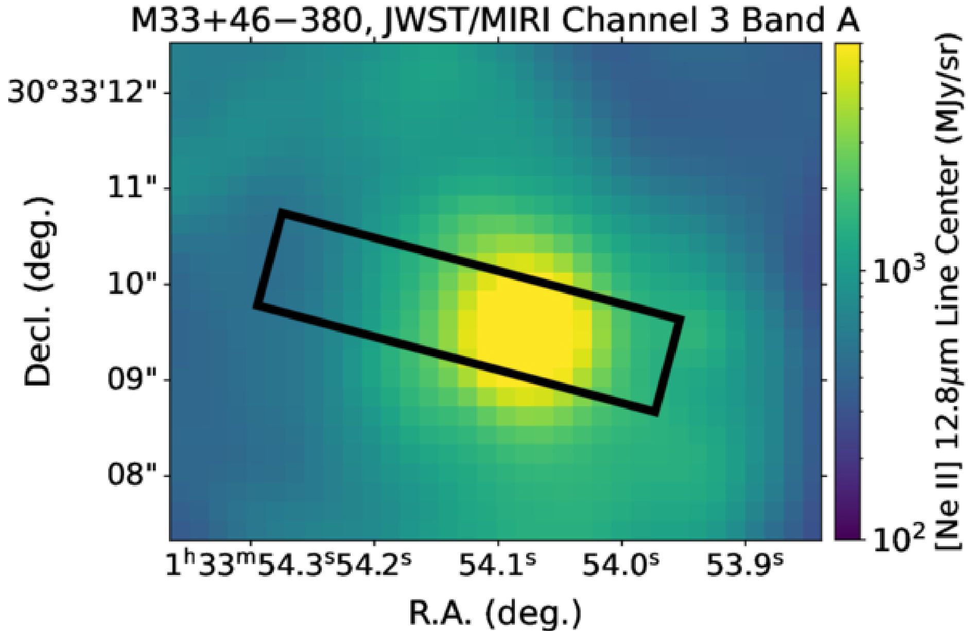
Figure 1. from Noah S. J. Rogers et al 2026 Astrophys. J. Lett. 1003 doi:10.3847/2041-8213/ae66f0 https://dx.doi.org/10.3847/2041-8213/ae66f0 © 2026. The Author(s). Published by the American Astronomical Society.
