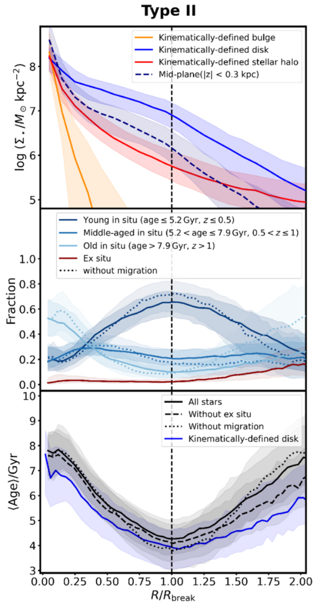
Figure 5. from Liufei Chen et al 2026 Astrophys. J. Lett. 1003 doi:10.3847/2041-8213/ae66ee https://dx.doi.org/10.3847/2041-8213/ae66ee © 2026. The Author(s). Published by the American Astronomical Society.
