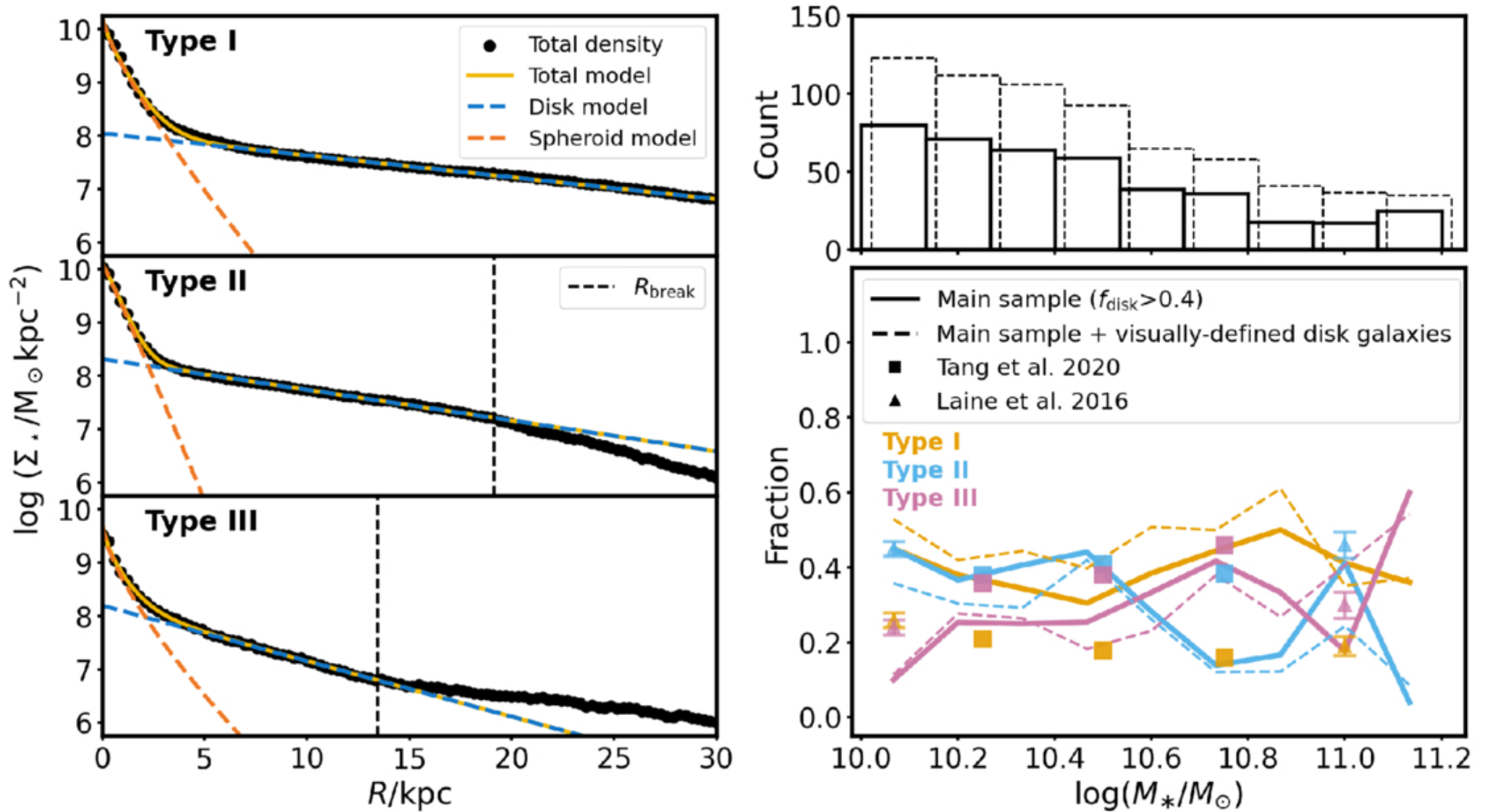
Figure 1. from Liufei Chen et al 2026 Astrophys. J. Lett. 1003 doi:10.3847/2041-8213/ae66ee https://dx.doi.org/10.3847/2041-8213/ae66ee © 2026. The Author(s). Published by the American Astronomical Society.
