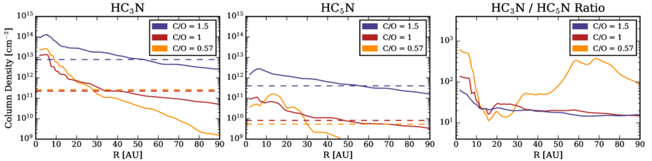
Figure 3. from Steven C. Wampler et al 2026 Astrophys. J. Lett. 1003 doi:10.3847/2041-8213/ae66e5 https://dx.doi.org/10.3847/2041-8213/ae66e5 © 2026. The Author(s). Published by the American Astronomical Society.
