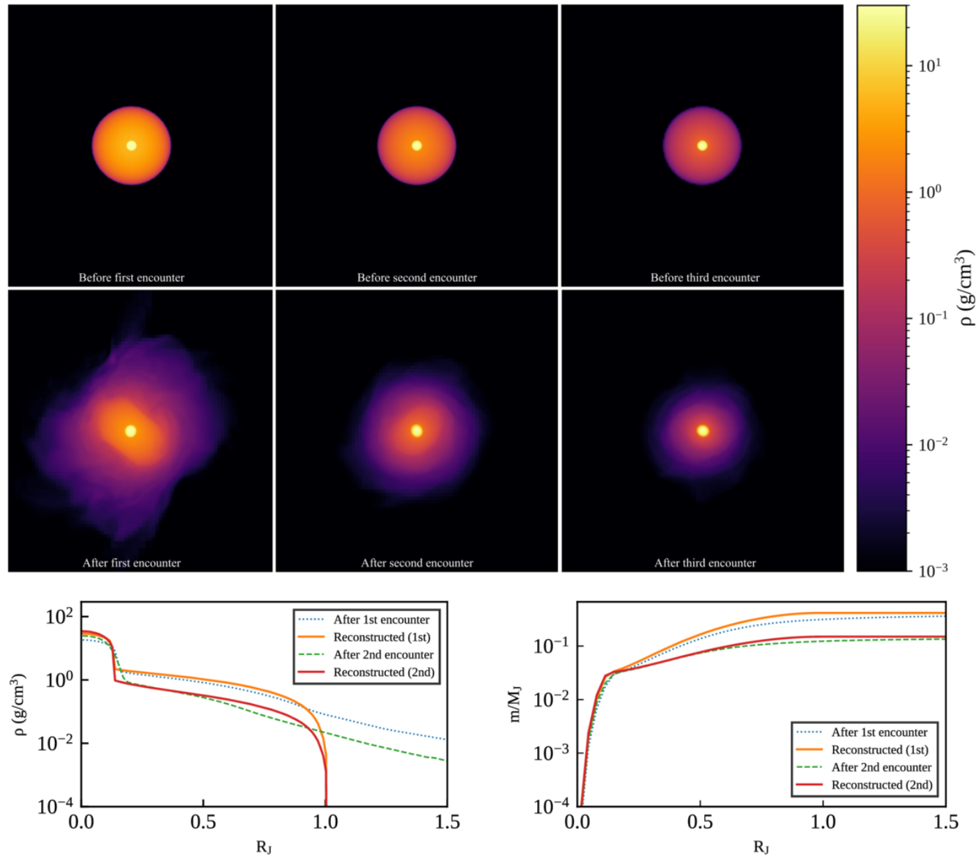
Figure 2. from Qianli Fan et al 2026 Astrophys. J. Lett. 1003 doi:10.3847/2041-8213/ae6659 https://dx.doi.org/10.3847/2041-8213/ae6659 © 2026. The Author(s). Published by the American Astronomical Society.
