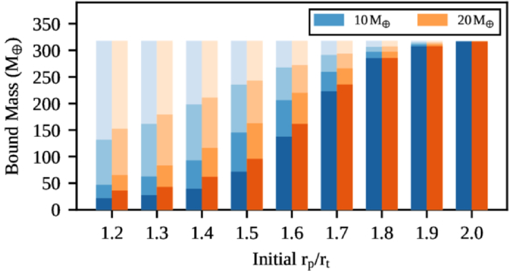
Figure 1. from Qianli Fan et al 2026 Astrophys. J. Lett. 1003 doi:10.3847/2041-8213/ae6659 https://dx.doi.org/10.3847/2041-8213/ae6659 © 2026. The Author(s). Published by the American Astronomical Society.
