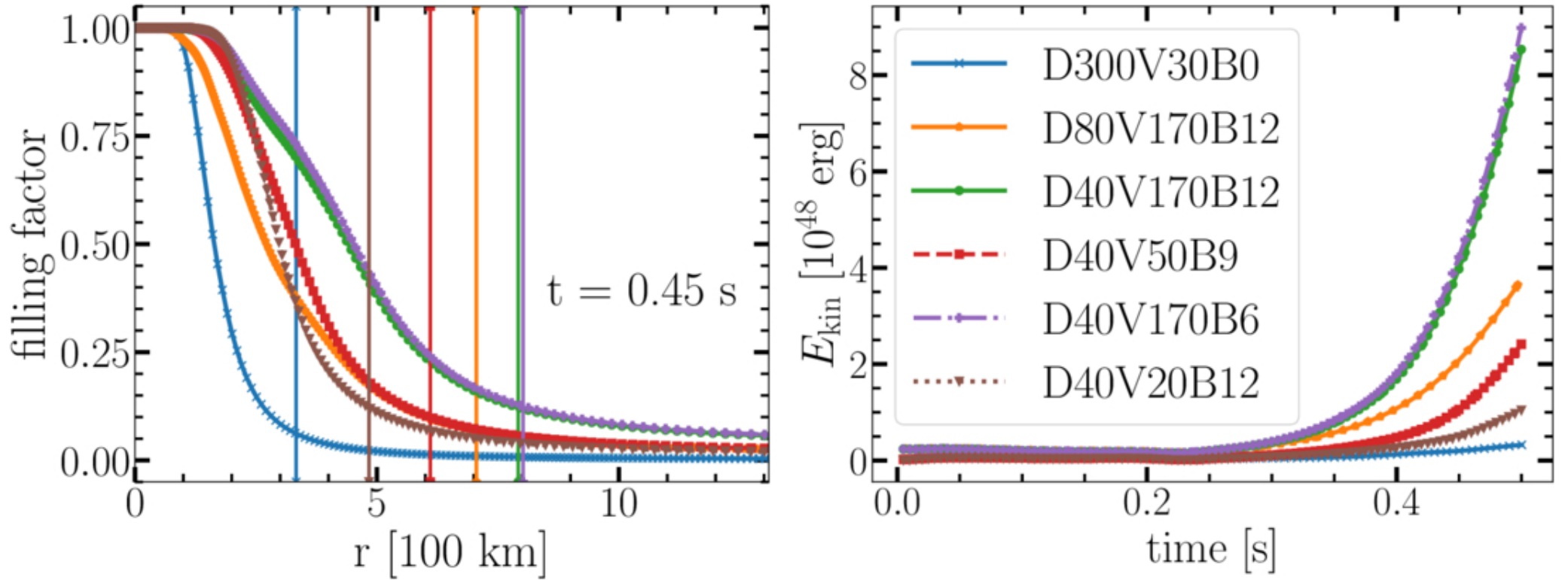
Figure 5. from S. Shiber et al 2026 Astrophys. J. Lett. 1003 doi:10.3847/2041-8213/ae664a https://dx.doi.org/10.3847/2041-8213/ae664a © 2026. The Author(s). Published by the American Astronomical Society.
