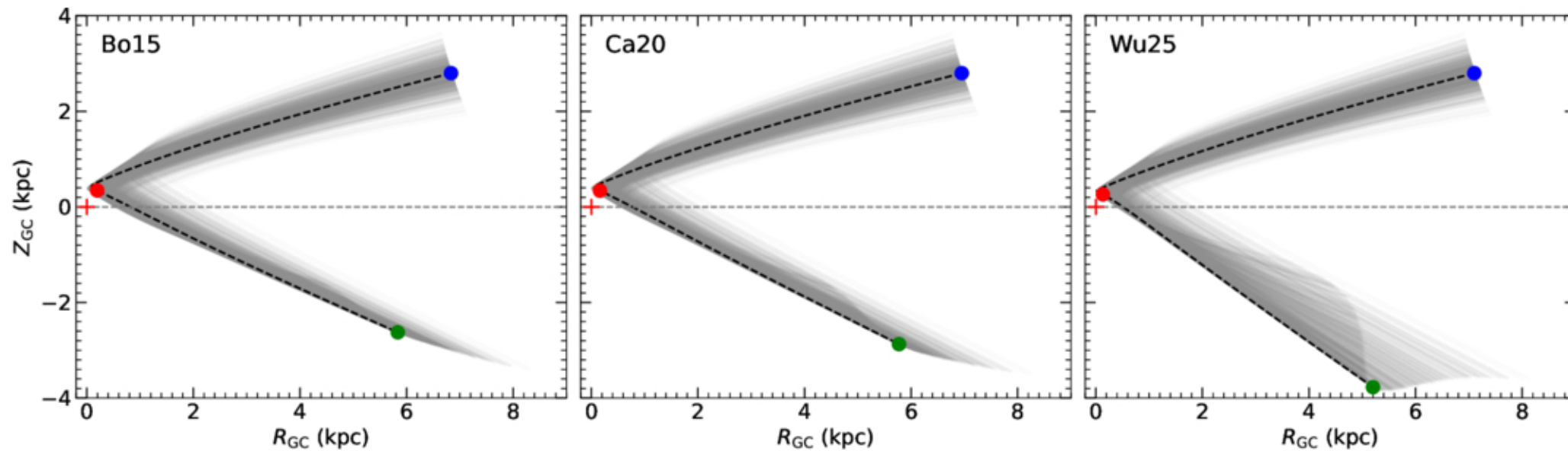
Figure 6. from Shunhong Deng et al 2026 Astrophys. J. Lett. 1003 doi:10.3847/2041-8213/ae6505 https://dx.doi.org/10.3847/2041-8213/ae6505 © 2026. The Author(s). Published by the American Astronomical Society.
