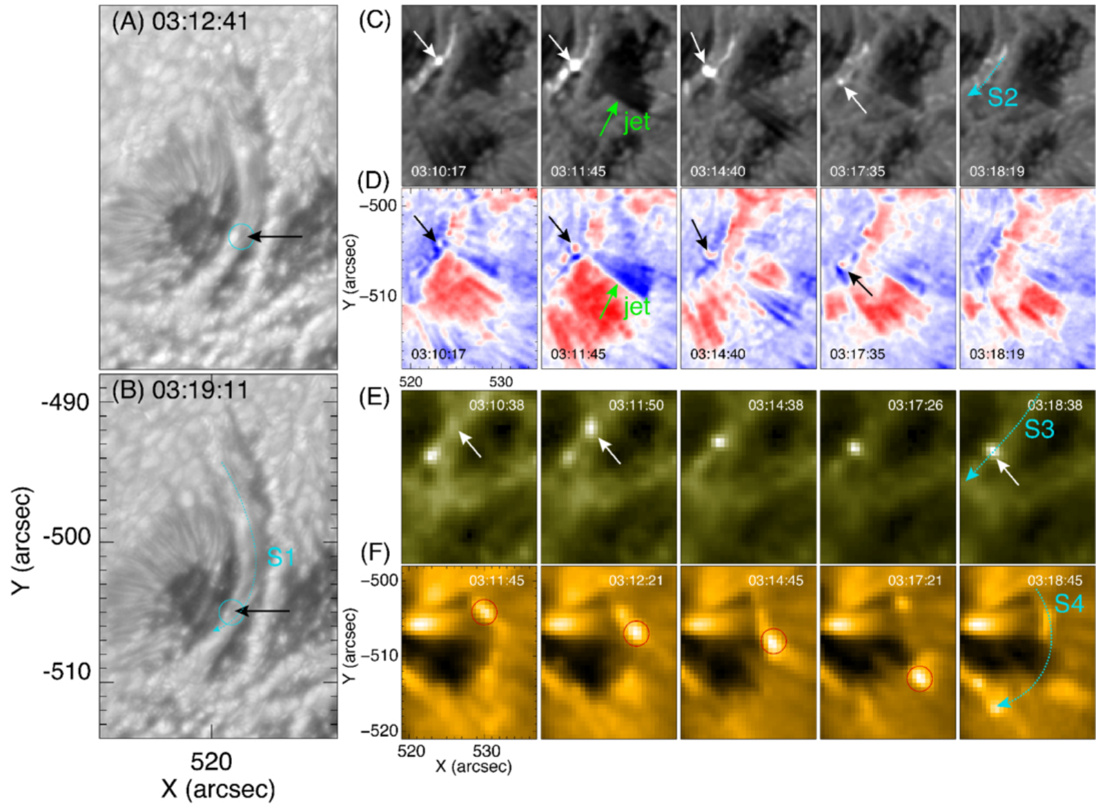
Figure 3. from Yadan Duan et al 2026 Astrophys. J. Lett. 1003 doi:10.3847/2041-8213/ae6340 https://dx.doi.org/10.3847/2041-8213/ae6340 © 2026. The Author(s). Published by the American Astronomical Society.
