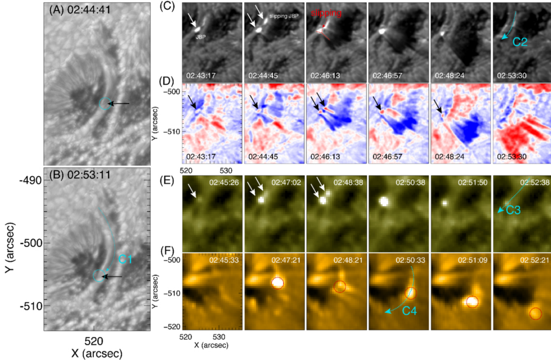
Figure 2. from Yadan Duan et al 2026 Astrophys. J. Lett. 1003 doi:10.3847/2041-8213/ae6340 https://dx.doi.org/10.3847/2041-8213/ae6340 © 2026. The Author(s). Published by the American Astronomical Society.
