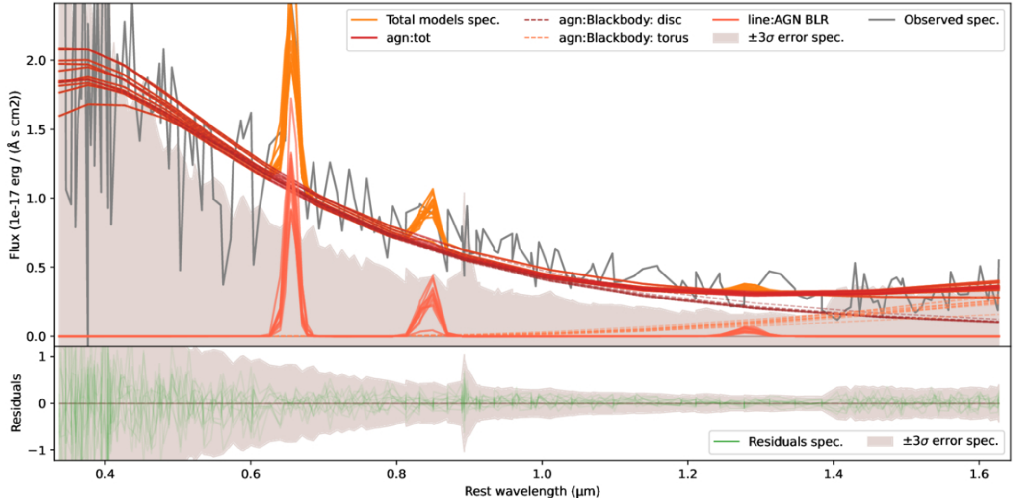
Figure 9. from Yuxing Zhong et al 2026 Astrophys. J. Lett. 1004 doi:10.3847/2041-8213/ae633b https://dx.doi.org/10.3847/2041-8213/ae633b © 2026. The Author(s). Published by the American Astronomical Society.
