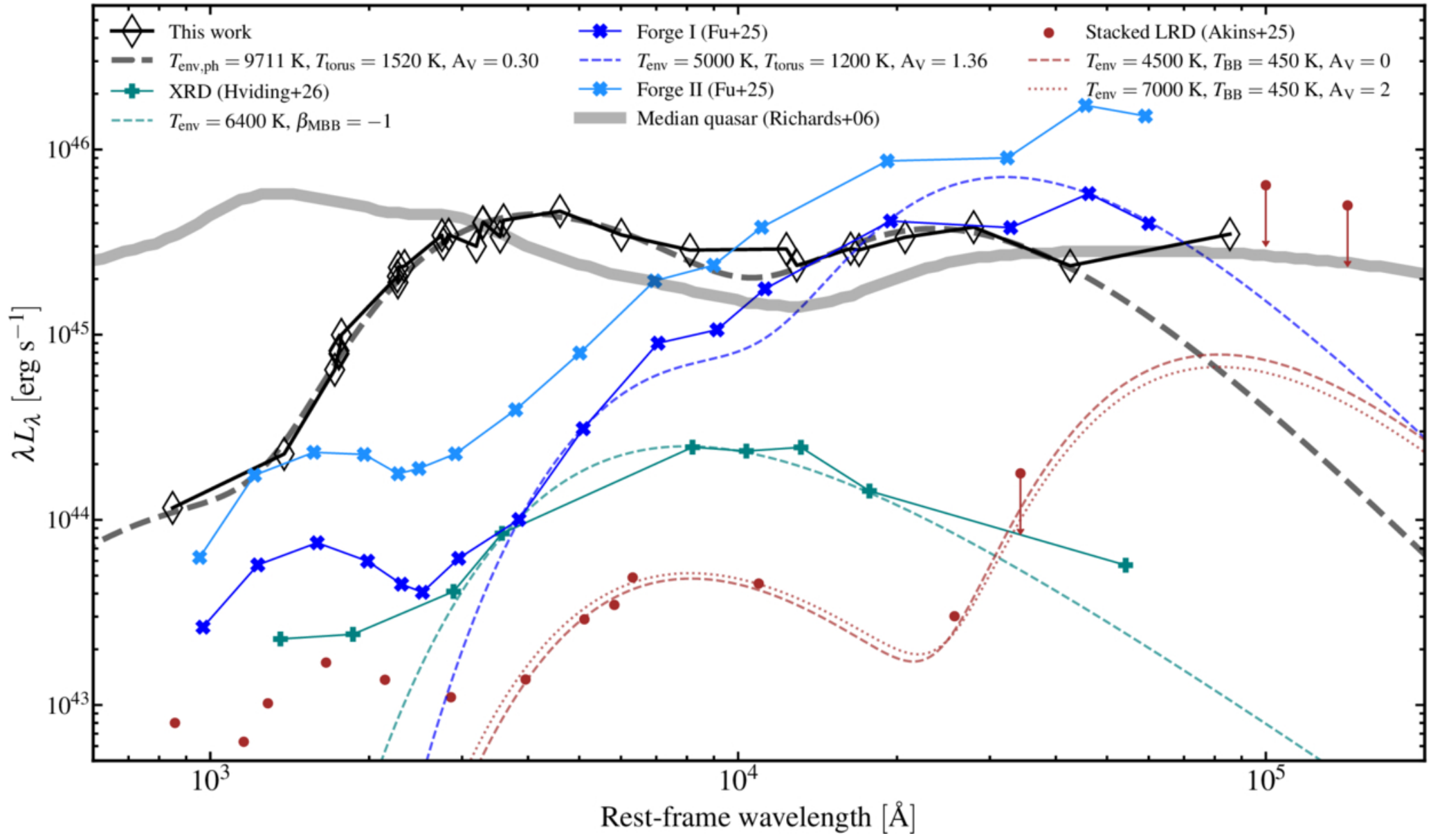
Figure 6. from Yuxing Zhong et al 2026 Astrophys. J. Lett. 1004 doi:10.3847/2041-8213/ae633b https://dx.doi.org/10.3847/2041-8213/ae633b © 2026. The Author(s). Published by the American Astronomical Society.
