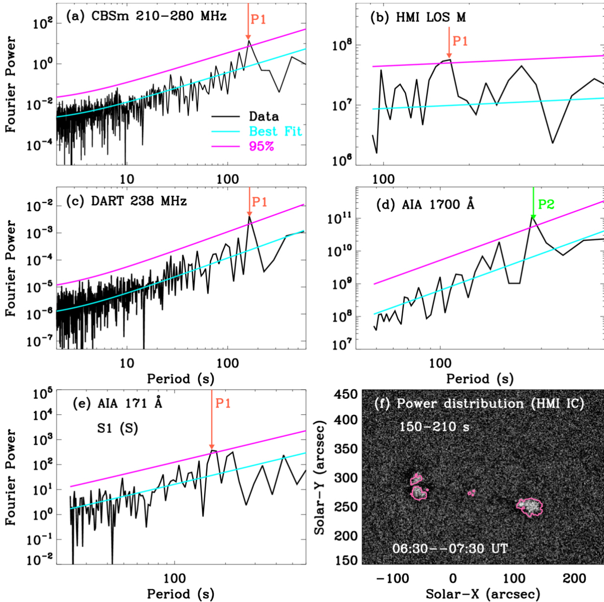
Figure 4. from Dong Li et al 2026 Astrophys. J. Lett. 1002 doi:10.3847/2041-8213/ae6271 https://dx.doi.org/10.3847/2041-8213/ae6271 © 2026. The Author(s). Published by the American Astronomical Society.
