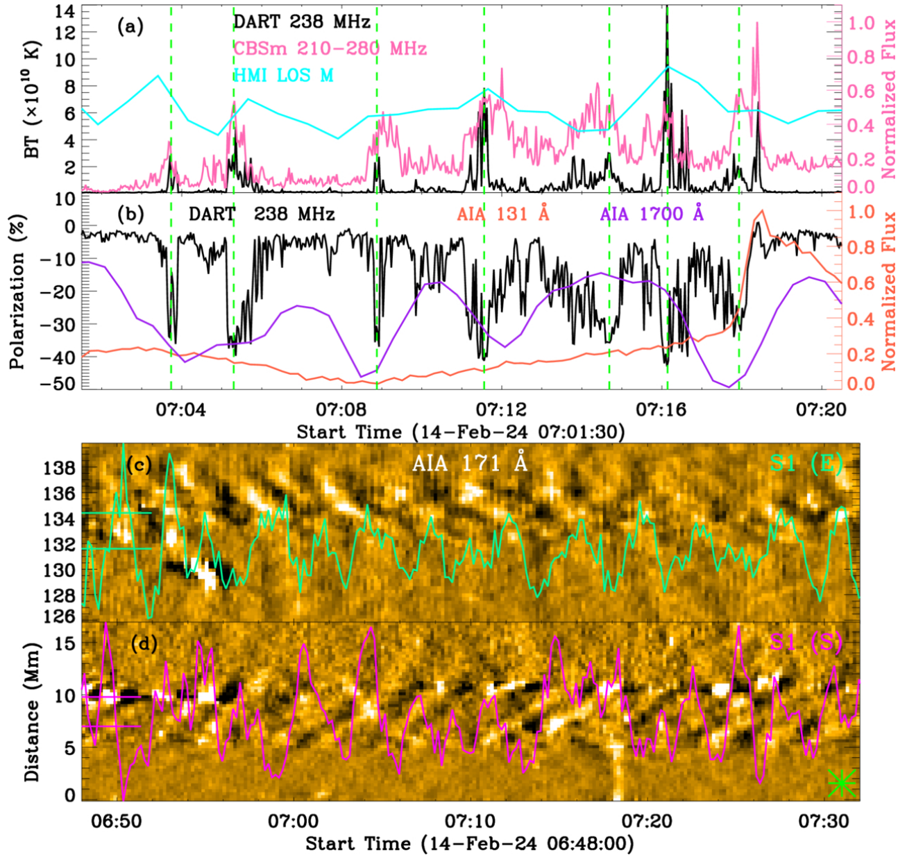
Figure 3. from Dong Li et al 2026 Astrophys. J. Lett. 1002 doi:10.3847/2041-8213/ae6271 https://dx.doi.org/10.3847/2041-8213/ae6271 © 2026. The Author(s). Published by the American Astronomical Society.
