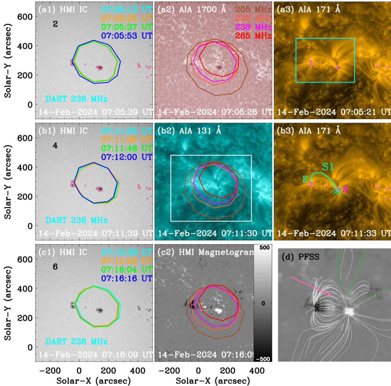
Figure 2. from Dong Li et al 2026 Astrophys. J. Lett. 1002 doi:10.3847/2041-8213/ae6271 https://dx.doi.org/10.3847/2041-8213/ae6271 © 2026. The Author(s). Published by the American Astronomical Society.
