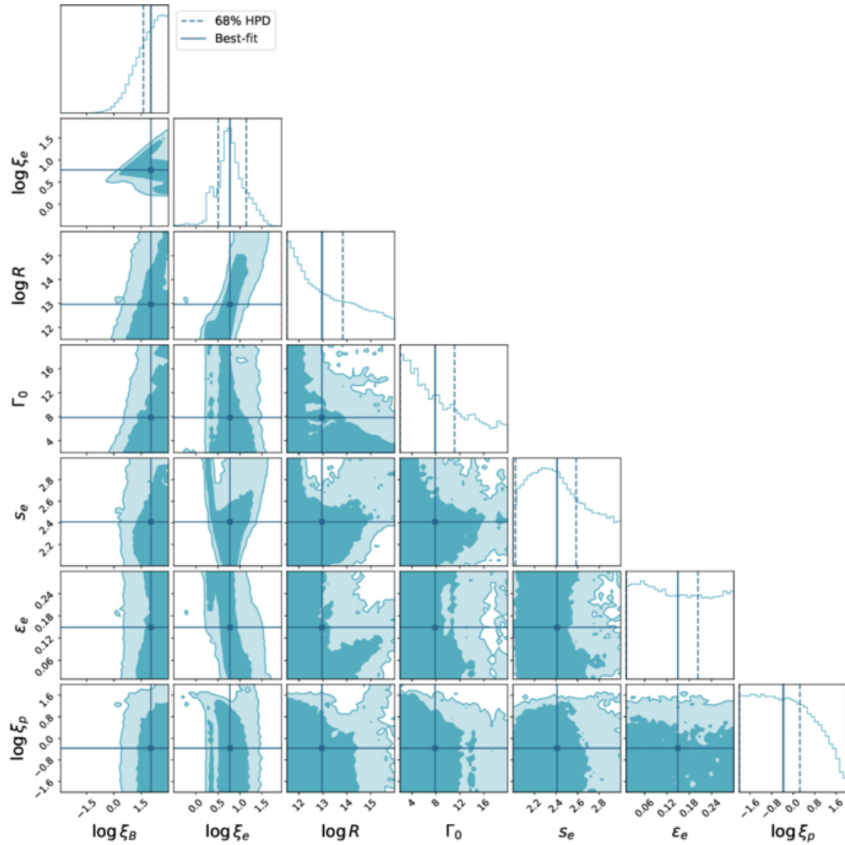
Figure 4. from Shiqi Yu et al 2026 Astrophys. J. Lett. 1002 doi:10.3847/2041-8213/ae626e https://dx.doi.org/10.3847/2041-8213/ae626e © 2026. The Author(s). Published by the American Astronomical Society.
