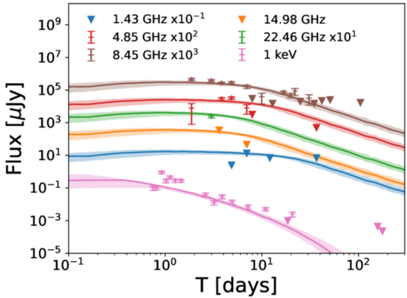
Figure 1. from Shiqi Yu et al 2026 Astrophys. J. Lett. 1002 doi:10.3847/2041-8213/ae626e https://dx.doi.org/10.3847/2041-8213/ae626e © 2026. The Author(s). Published by the American Astronomical Society.
