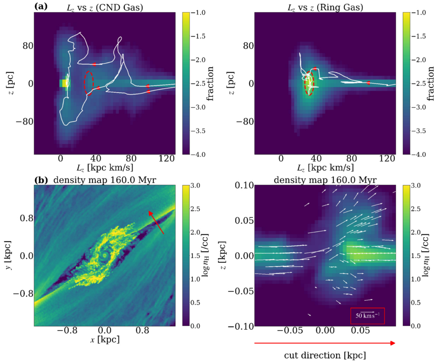
Figure 4. from Kotaro Kobayashi et al 2026 Astrophys. J. Lett. 1002 doi:10.3847/2041-8213/ae6262 https://dx.doi.org/10.3847/2041-8213/ae6262 © 2026. The Author(s). Published by the American Astronomical Society.
