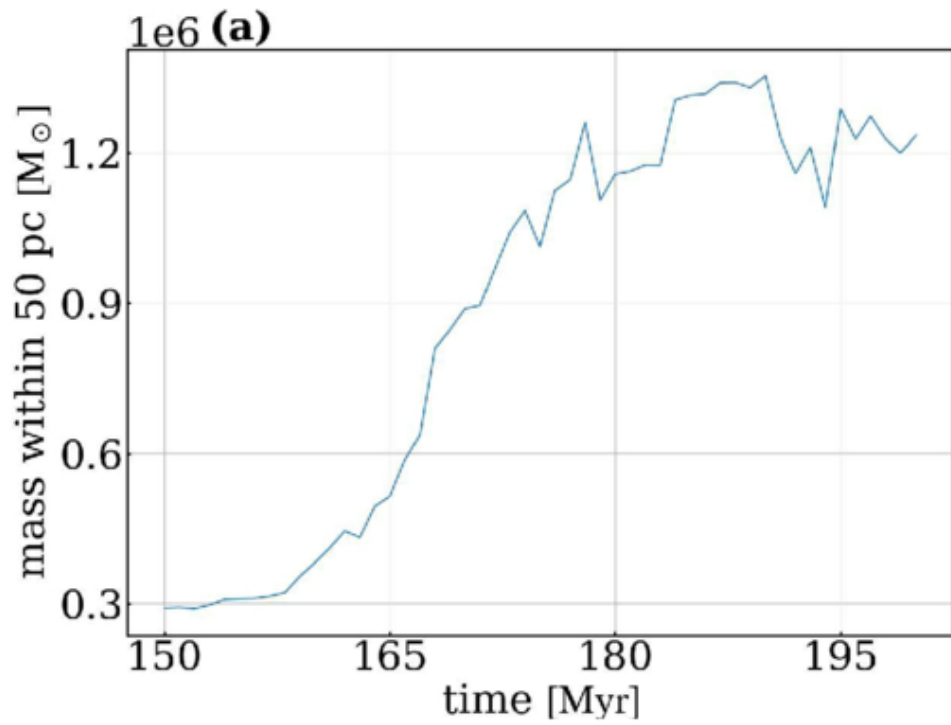
Figure 3. from Kotaro Kobayashi et al 2026 Astrophys. J. Lett. 1002 doi:10.3847/2041-8213/ae6262 https://dx.doi.org/10.3847/2041-8213/ae6262 © 2026. The Author(s). Published by the American Astronomical Society.
