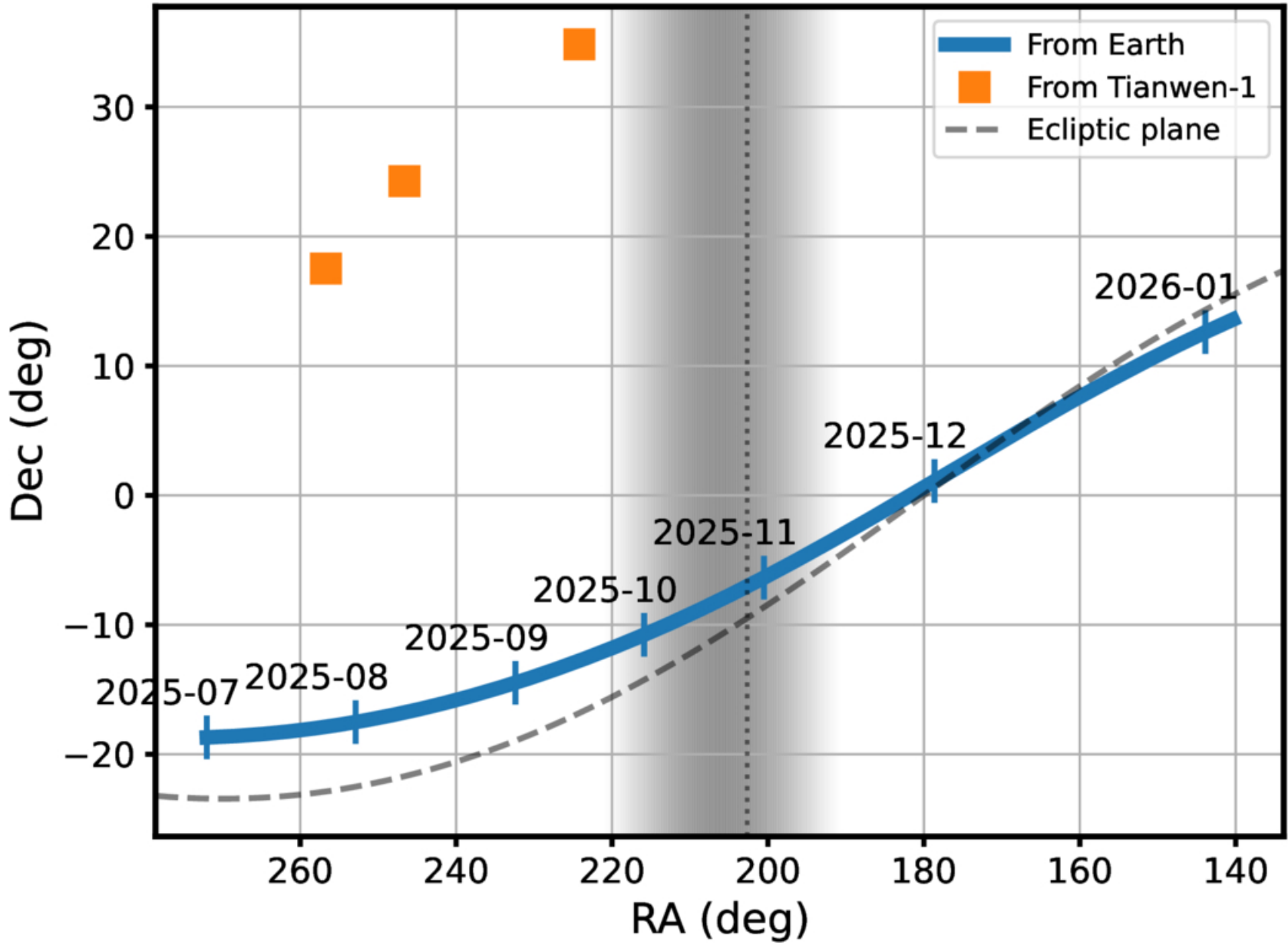
Figure 1. from Xin Ren et al 2026 Astrophys. J. Lett. 1003 doi:10.3847/2041-8213/ae61b3 https://dx.doi.org/10.3847/2041-8213/ae61b3 © 2026. The Author(s). Published by the American Astronomical Society.
