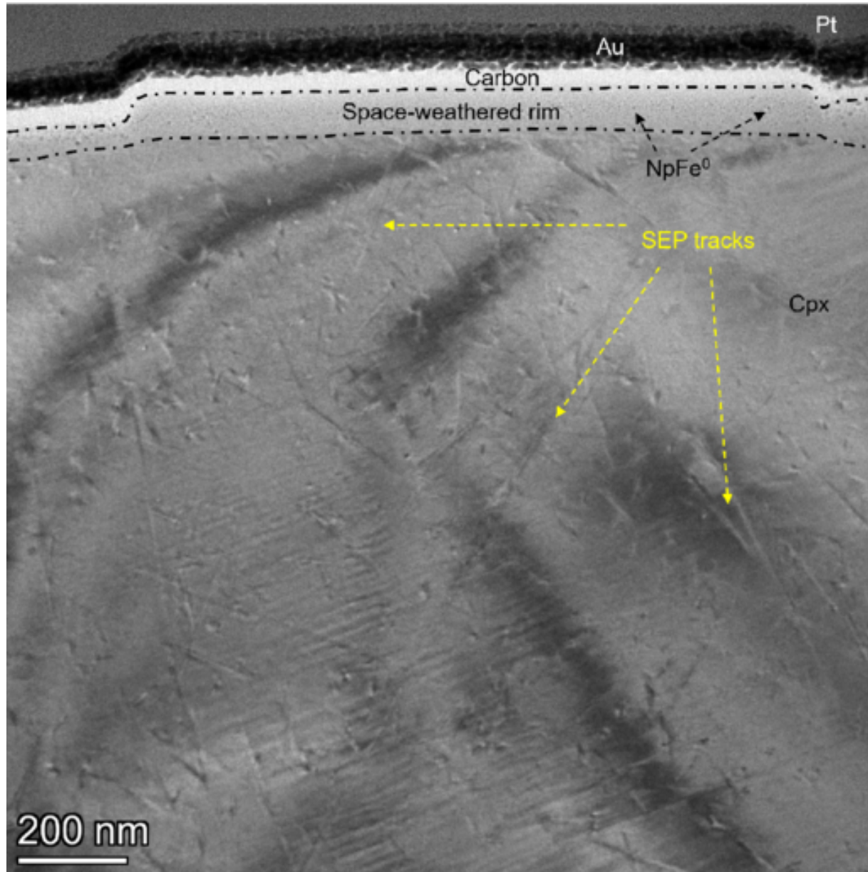
Figure A2. from Chenkun Sun et al 2026 Astrophys. J. Lett. 1002 doi:10.3847/2041-8213/ae61b2 https://dx.doi.org/10.3847/2041-8213/ae61b2 © 2026. The Author(s). Published by the American Astronomical Society.
