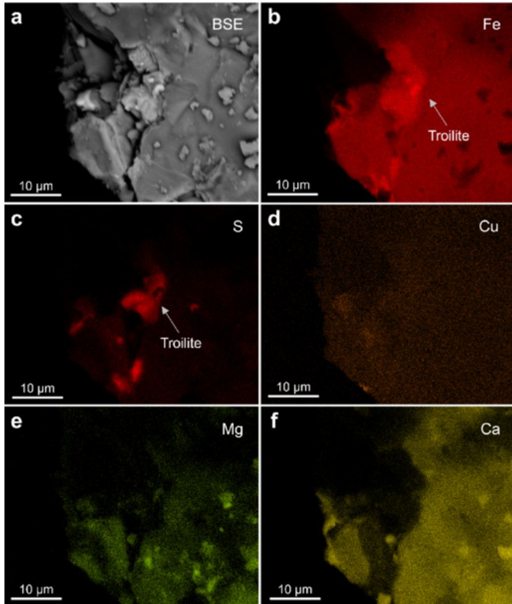
Figure A1. from Chenkun Sun et al 2026 Astrophys. J. Lett. 1002 doi:10.3847/2041-8213/ae61b2 https://dx.doi.org/10.3847/2041-8213/ae61b2 © 2026. The Author(s). Published by the American Astronomical Society.
