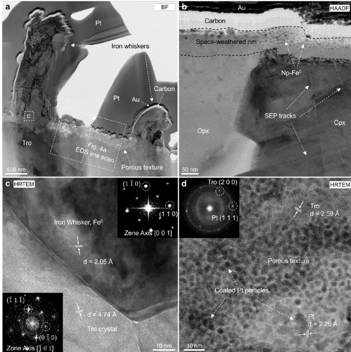
Figure 3. from Chenkun Sun et al 2026 Astrophys. J. Lett. 1002 doi:10.3847/2041-8213/ae61b2 https://dx.doi.org/10.3847/2041-8213/ae61b2 © 2026. The Author(s). Published by the American Astronomical Society.
