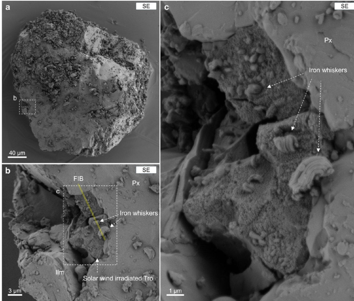
Figure 1. from Chenkun Sun et al 2026 Astrophys. J. Lett. 1002 doi:10.3847/2041-8213/ae61b2 https://dx.doi.org/10.3847/2041-8213/ae61b2 © 2026. The Author(s). Published by the American Astronomical Society.
