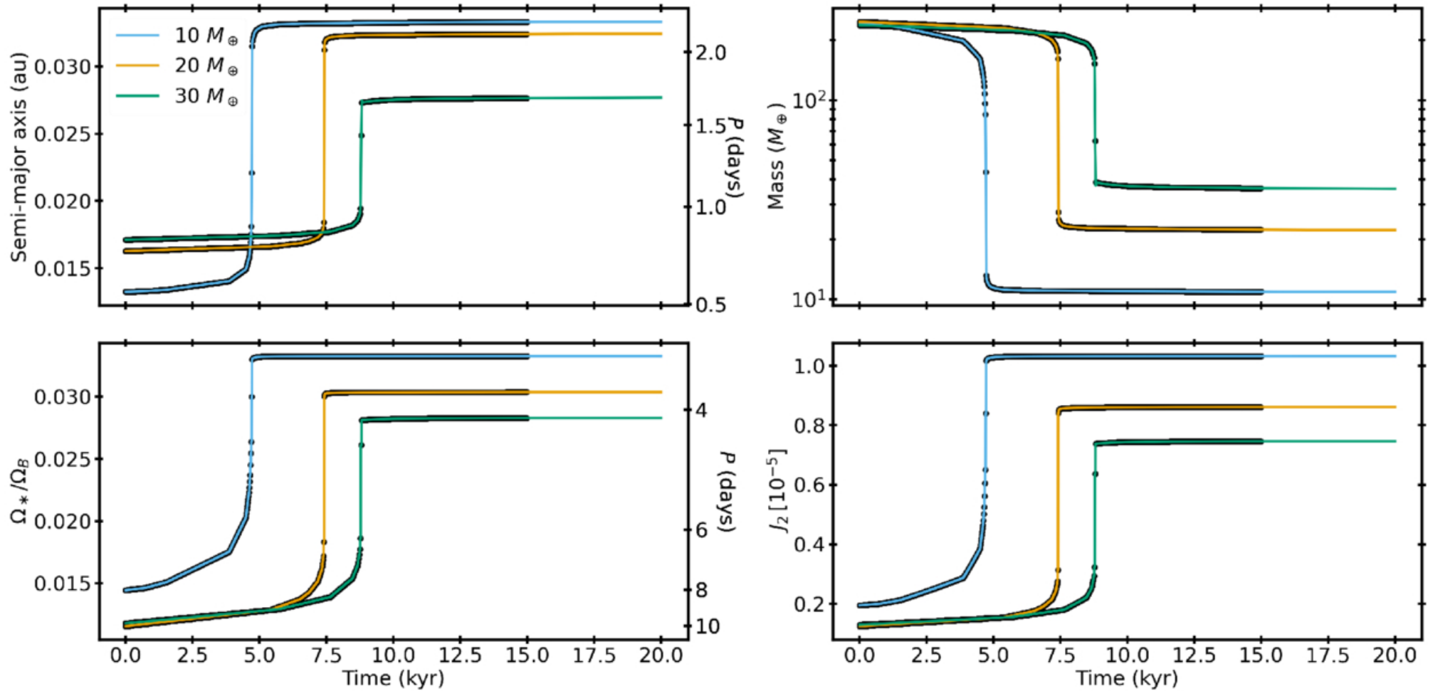
Figure 1. from Donald Liveoak et al 2026 Astrophys. J. Lett. 1002 doi:10.3847/2041-8213/ae61b1 https://dx.doi.org/10.3847/2041-8213/ae61b1 © 2026. The Author(s). Published by the American Astronomical Society.
