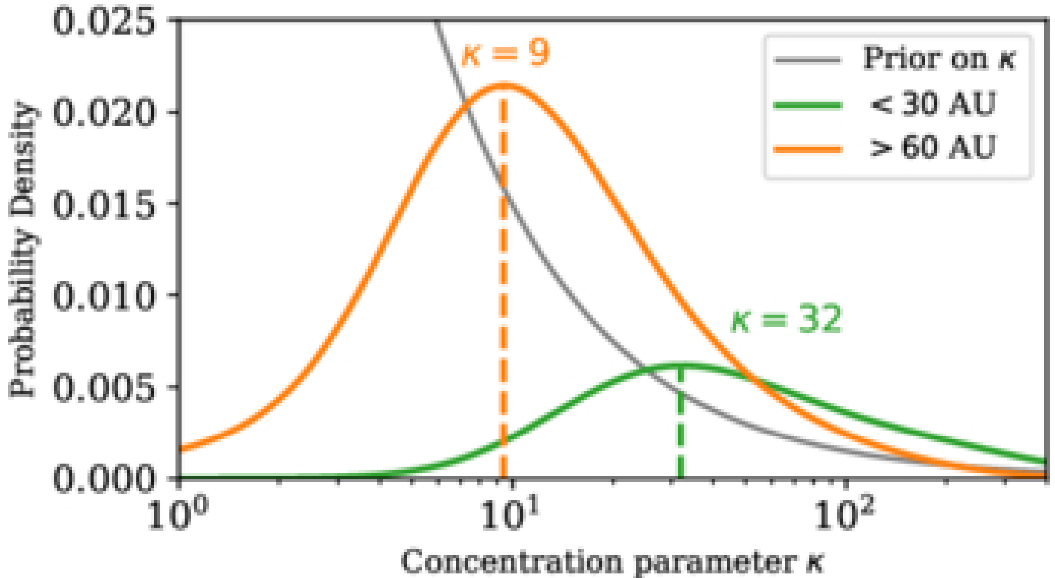
Figure 9. from Michael Poon et al 2026 Astrophys. J. Lett. 1002 doi:10.3847/2041-8213/ae61af https://dx.doi.org/10.3847/2041-8213/ae61af © 2026. The Author(s). Published by the American Astronomical Society.
