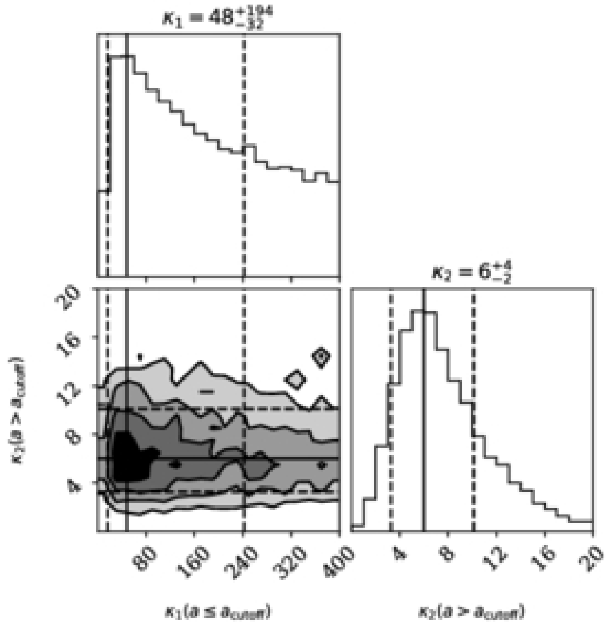
Figure 11. from Michael Poon et al 2026 Astrophys. J. Lett. 1002 doi:10.3847/2041-8213/ae61af https://dx.doi.org/10.3847/2041-8213/ae61af © 2026. The Author(s). Published by the American Astronomical Society.
