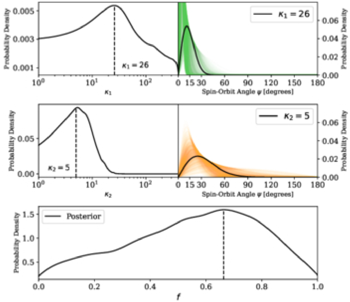
Figure 10. from Michael Poon et al 2026 Astrophys. J. Lett. 1002 doi:10.3847/2041-8213/ae61af https://dx.doi.org/10.3847/2041-8213/ae61af © 2026. The Author(s). Published by the American Astronomical Society.
