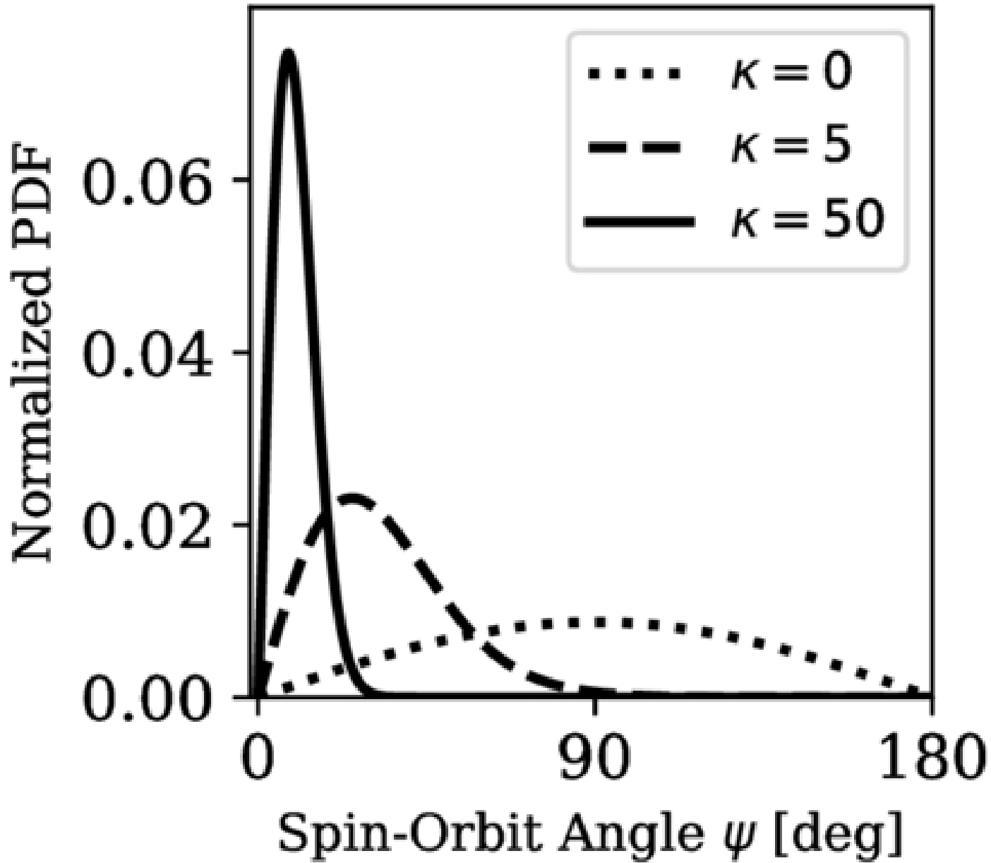
Figure 1. from Michael Poon et al 2026 Astrophys. J. Lett. 1002 doi:10.3847/2041-8213/ae61af https://dx.doi.org/10.3847/2041-8213/ae61af © 2026. The Author(s). Published by the American Astronomical Society.
