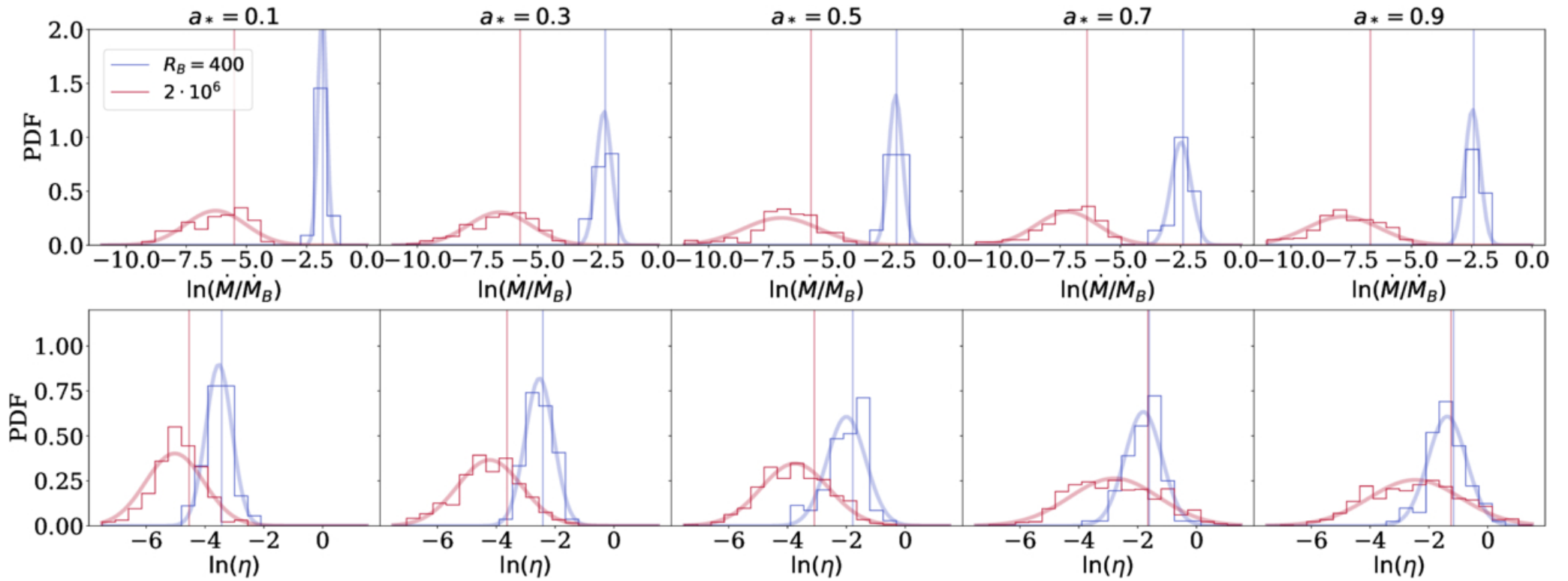
Figure 3. from Hyerin Cho et al 2026 Astrophys. J. Lett. 1002 doi:10.3847/2041-8213/ae61ae https://dx.doi.org/10.3847/2041-8213/ae61ae © 2026. The Author(s). Published by the American Astronomical Society.
