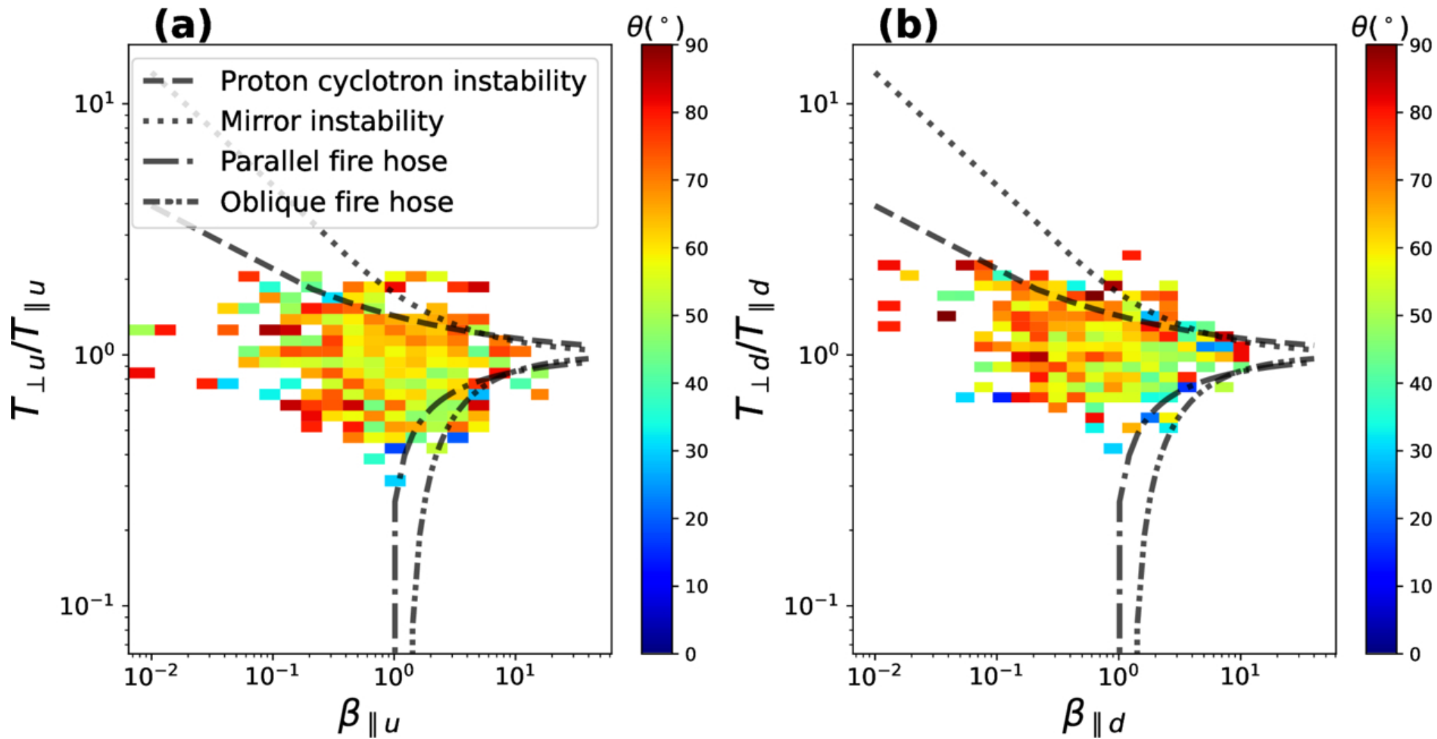
Figure 6. from Zeping Jin et al 2026 Astrophys. J. Lett. 1002 doi:10.3847/2041-8213/ae6067 https://dx.doi.org/10.3847/2041-8213/ae6067 © 2026. The Author(s). Published by the American Astronomical Society.
