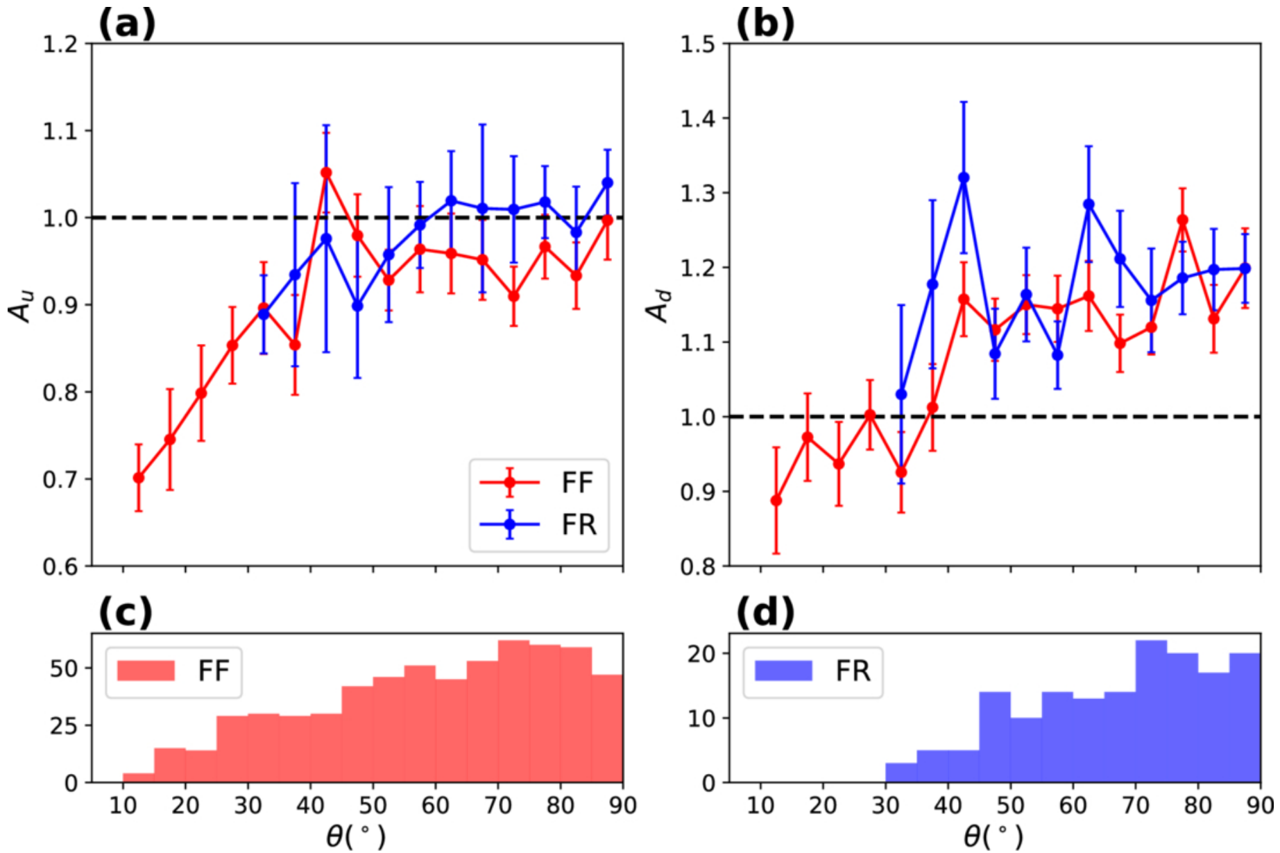
Figure 1. from Zeping Jin et al 2026 Astrophys. J. Lett. 1002 doi:10.3847/2041-8213/ae6067 https://dx.doi.org/10.3847/2041-8213/ae6067 © 2026. The Author(s). Published by the American Astronomical Society.
