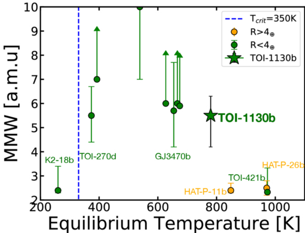
Figure 7. from Saugata Barat et al 2026 Astrophys. J. Lett. 1002 doi:10.3847/2041-8213/ae5f8b https://dx.doi.org/10.3847/2041-8213/ae5f8b © 2026. The Author(s). Published by the American Astronomical Society.
