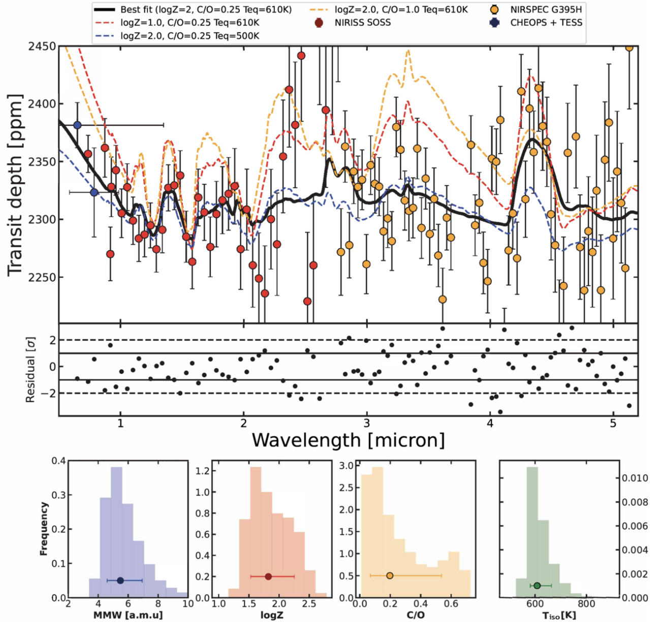
Figure 3. from Saugata Barat et al 2026 Astrophys. J. Lett. 1002 doi:10.3847/2041-8213/ae5f8b https://dx.doi.org/10.3847/2041-8213/ae5f8b © 2026. The Author(s). Published by the American Astronomical Society.
