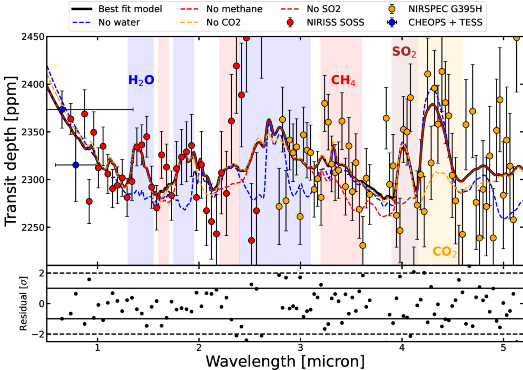
Figure 2. from Saugata Barat et al 2026 Astrophys. J. Lett. 1002 doi:10.3847/2041-8213/ae5f8b https://dx.doi.org/10.3847/2041-8213/ae5f8b © 2026. The Author(s). Published by the American Astronomical Society.
