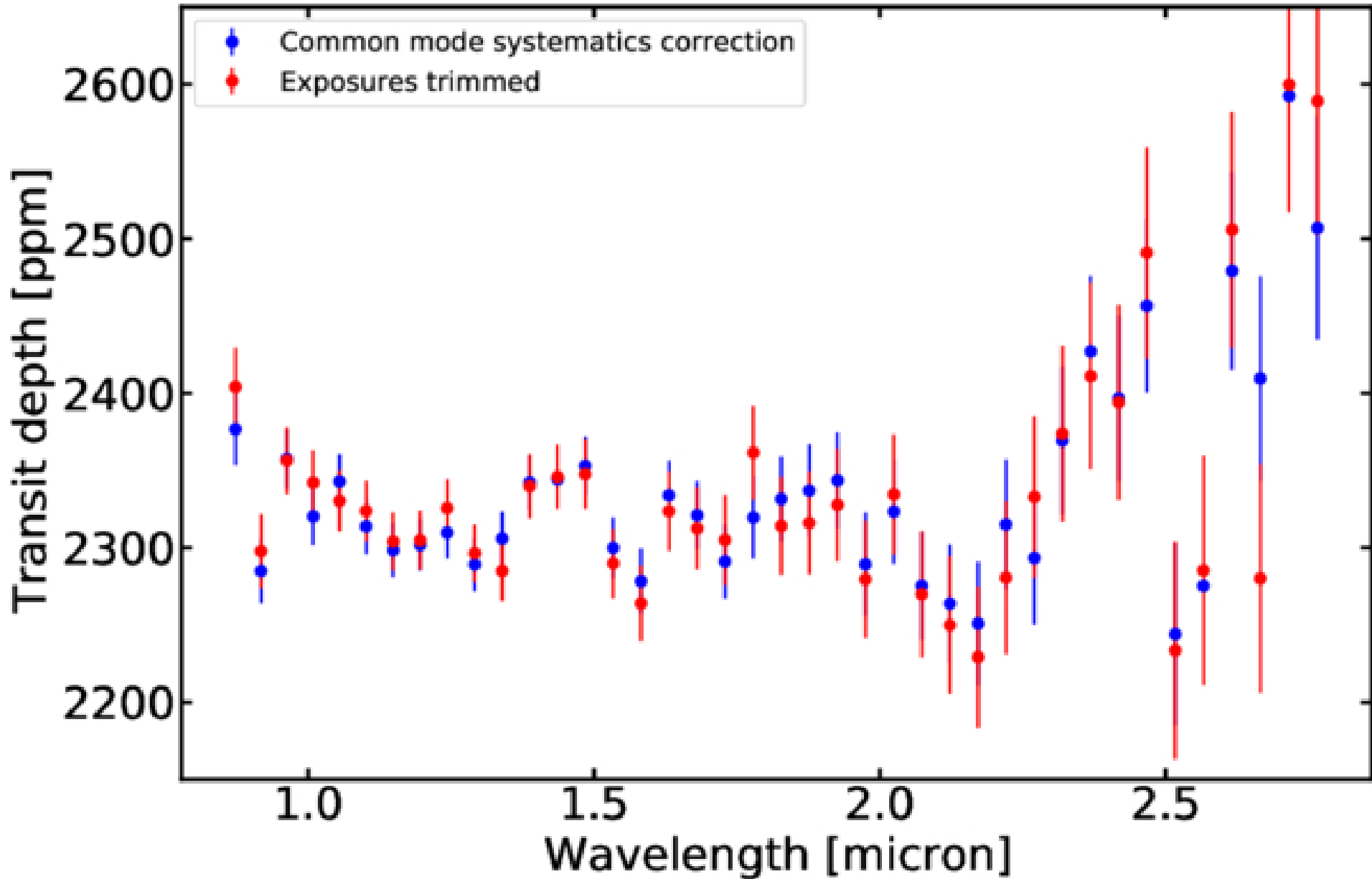
Figure B3. from Saugata Barat et al 2026 Astrophys. J. Lett. 1002 doi:10.3847/2041-8213/ae5f8b https://dx.doi.org/10.3847/2041-8213/ae5f8b © 2026. The Author(s). Published by the American Astronomical Society.
