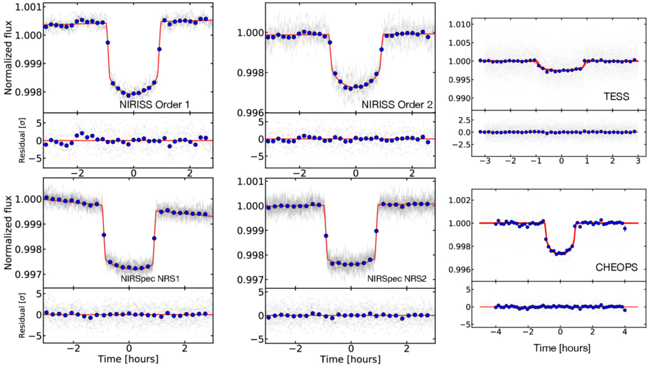
Figure 1. from Saugata Barat et al 2026 Astrophys. J. Lett. 1002 doi:10.3847/2041-8213/ae5f8b https://dx.doi.org/10.3847/2041-8213/ae5f8b © 2026. The Author(s). Published by the American Astronomical Society.
