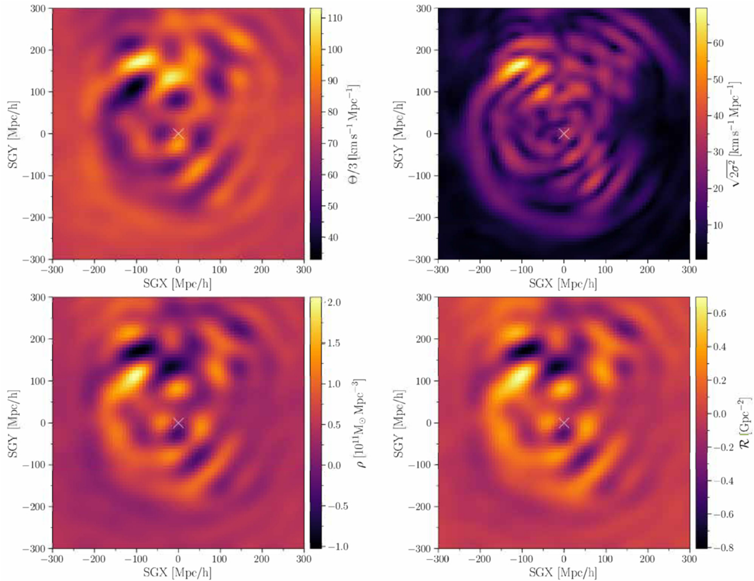
Figure 1. from Marco Galoppo et al 2026 Astrophys. J. Lett. 1002 doi:10.3847/2041-8213/ae5f73 https://dx.doi.org/10.3847/2041-8213/ae5f73 © 2026. The Author(s). Published by the American Astronomical Society.
